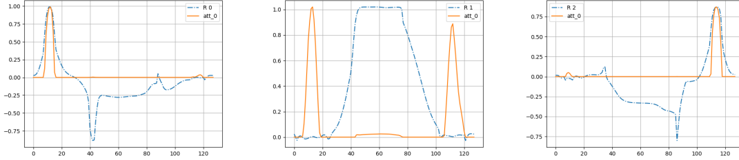
Figure 16: Attention weights ( A_t(i) ) for the BME dataset (orange curve, plain line). The corresponding reference vector R_u is presented in blue dotted line. Time is the horizontal axis.
