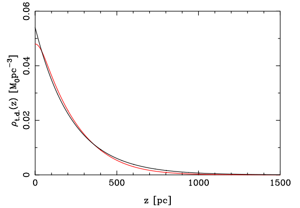
Fig. 10. Vertical mass density of the stellar thin discs from the Besan on model (red line) fitted with an exponential of scale height h = 229 pc (black line).
