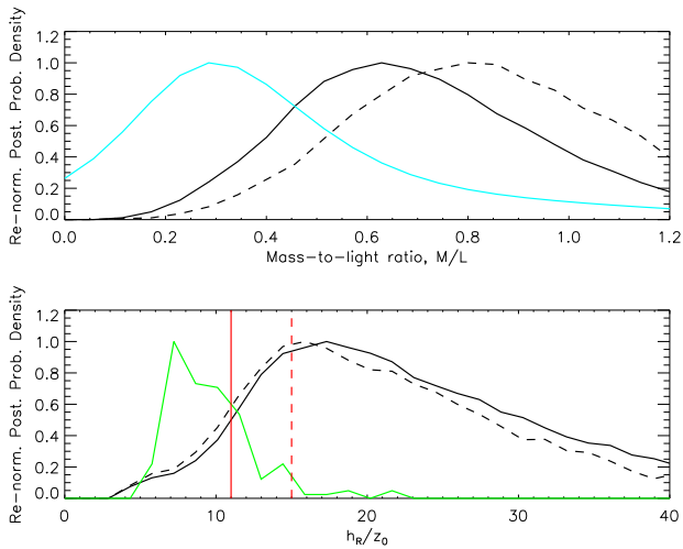
Figure 26. Top panel: superposition of the re-normalized posterior probability densities of fitted mass-to-light ratios, using a \text{sech}^2 function to describe the vertical distribution of the stellar disk, for the 30 galaxies in the DiskMass sample. The black solid curve corresponds to the \gamma = 1 interpolating function and the black dashed curve to \gamma = 2 . The distribution found by the DMS, with an exponential vertical distribution, uses a turquoise curve and is just shown for reference. Bottom panel: superposition of the re-normalized posterior probability density of fitted scalelength to vertical scaleheight, using a \text{sech}^2 distribution, for the 30 galaxies in the DiskMass sample. The black solid curve corresponds to the \gamma = 1 interpolating function and the black dashed curve to \gamma = 2 . The green curve is the probability density of the sample of 153 galaxies from Bizyaev & Mitronova (2002). The vertical solid red line represents the value of h_R/z_0 at which the sample of Mosenkov et al. (2010) begins to decline from a previously flat value. The dashed red line represents where the probability density of Mosenkov et al. (2010) drops to zero. Using a \text{sech}^2 distribution does not improve the ability of MOND to fit the DMS without decreased scaleheights.
