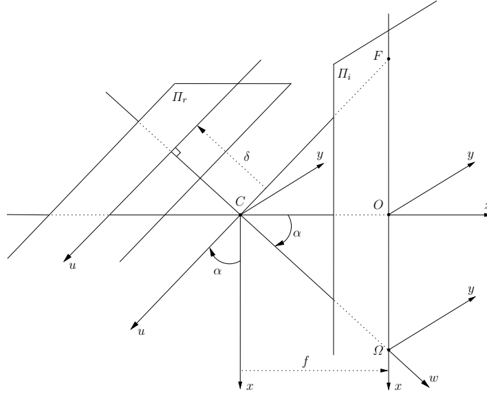
Fig. 1. Representation of the photographic bench.
