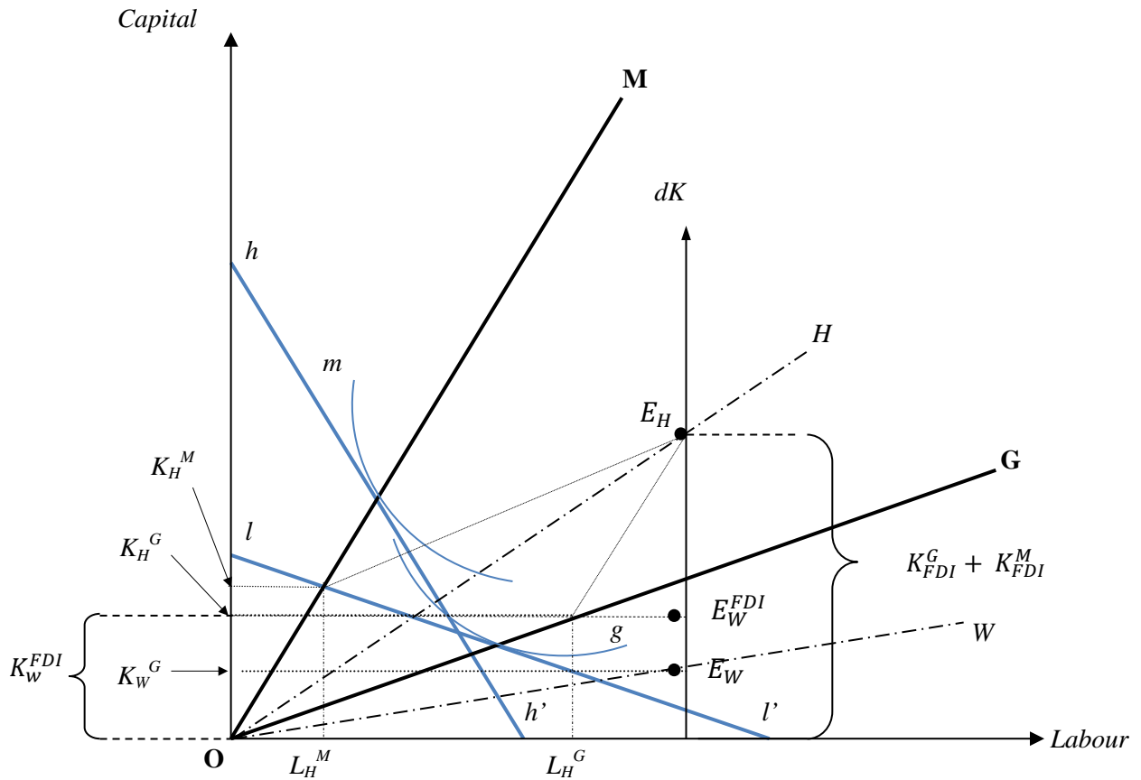
Figure 1: Lerner diagram 2 countries x 2 factors x 2 goods with vertical FDI
