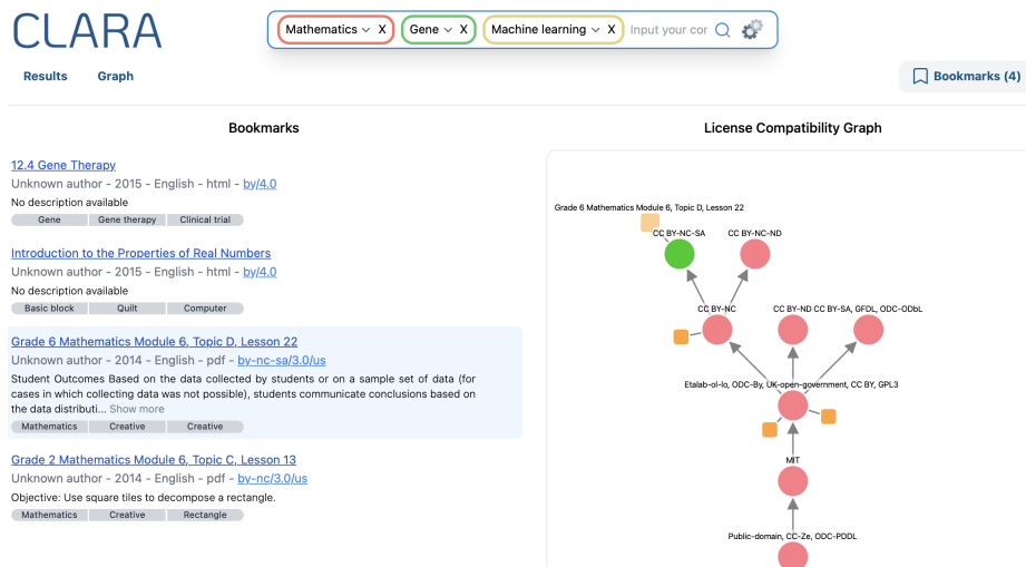
Fig. 1. Screenshot of the CLARA search engine. It shows the compatibility graph of licences of some bookmarked ERs. The license in green can protect a new course mixing-up the bookmarked ERs.
