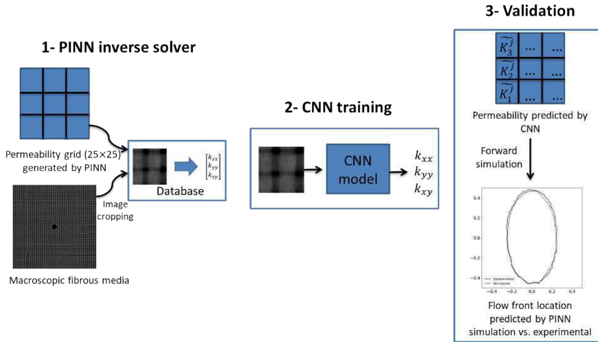
Figure 6: The full sequential training methodology to predict the permeability tensor field from textile images.
