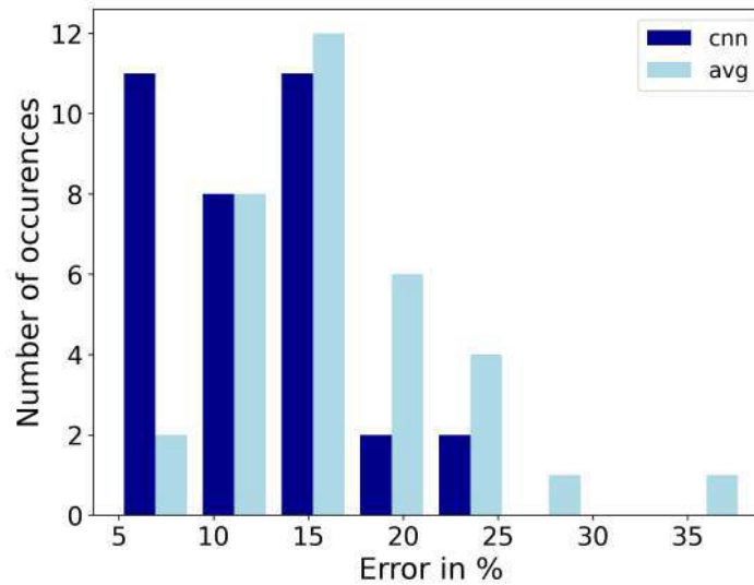
Figure 13: Histogram plot showing the number of occurrences in the y -axis and the mispredicted pixels error e_p measure in percentage in the x -axis for the simulation using CNN-predicted permeability and the simulation using the average permeability.
