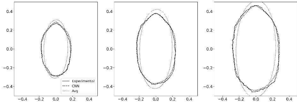
Figure 16: Flow front location at 3 different time instants of experiments number 24. The figures show the experimental flow front along with the simulated flow front using the CNN predicted permeability and the measured average permeability value.
