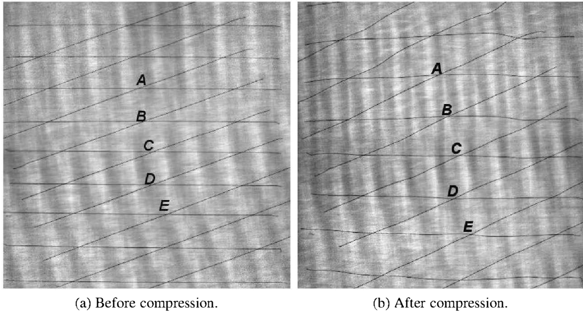
Figure 5. CT scan of \{0^\circ, 20^\circ, 0^\circ\} specimen
