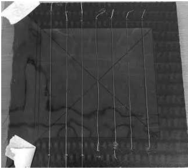
(a) Laying of copper wires along the fiber direction.
