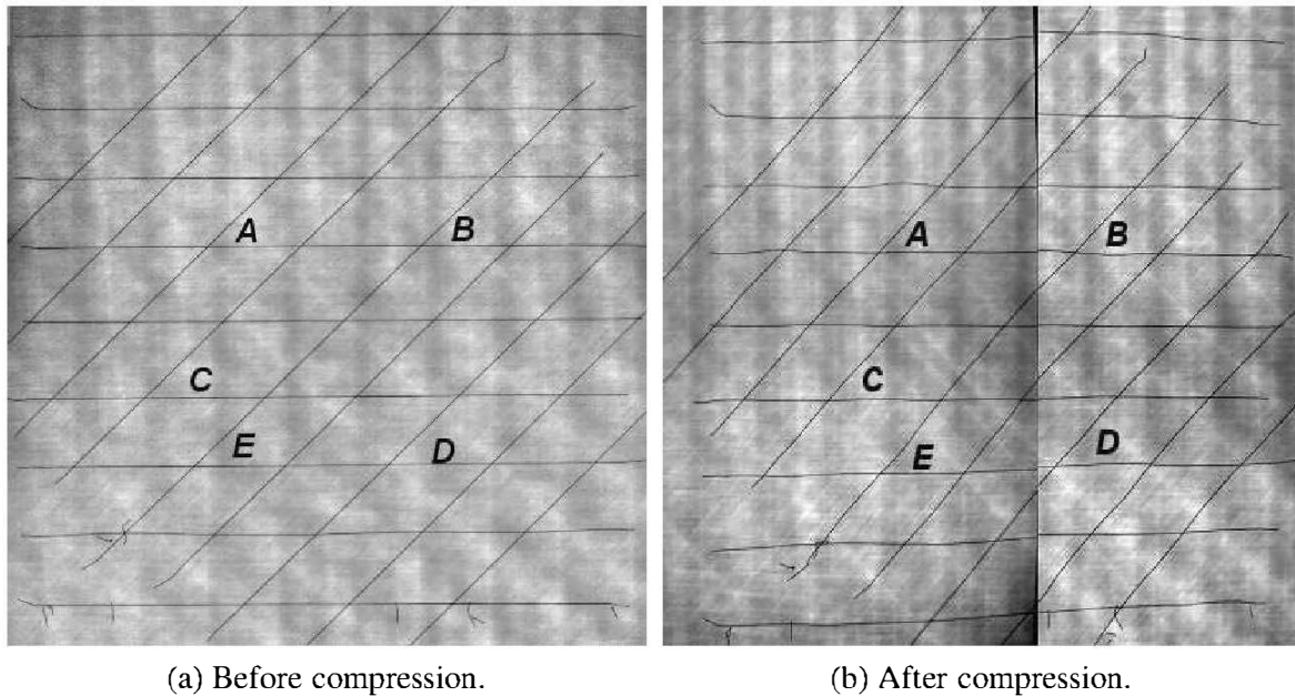
Figure 6. CT-scans of \{0^\circ, 45^\circ, 0^\circ\} specimen
