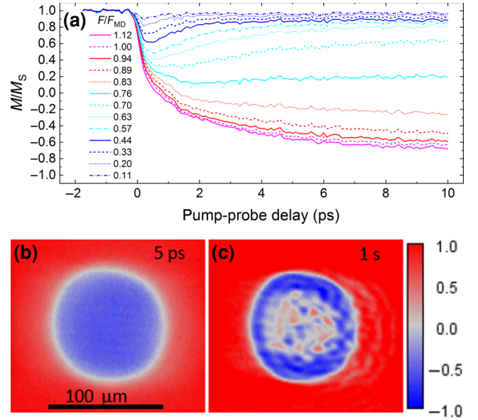
FIG. 4. (a) Magnetization dynamics in \alpha -Gd 18 Dy 4 Co 78 induced by s -polarized, 150-fs, 800-nm laser pulses of various fluences (given in multiples of F_{\text{MD}} = 5.9 mJ/cm 2 ) incident at approximately equal to 5°. Panels (b),(c) show normalized magnetization profiles 5 ps and 1 s after the excitation, respectively.
