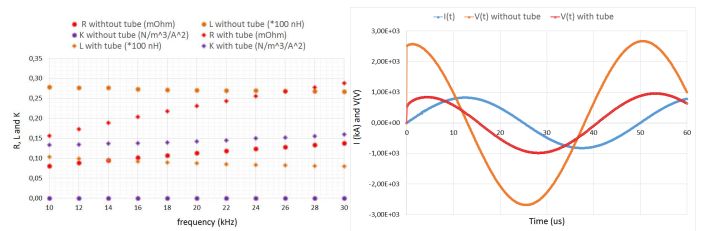
Figure 7. R, L and K v.s. \omega .
