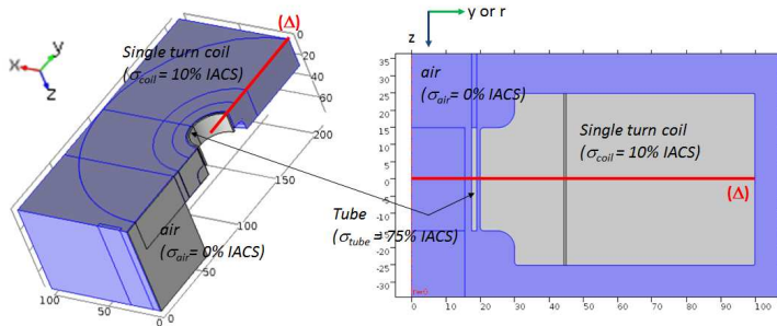
Figure 1. 3D and 2D Geometry.
