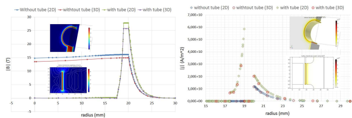
Figure 3. |B|(r) along (\Delta) @ I = 825 \text{ kA} @ \omega/2\pi = 20 \text{ kHz} .
