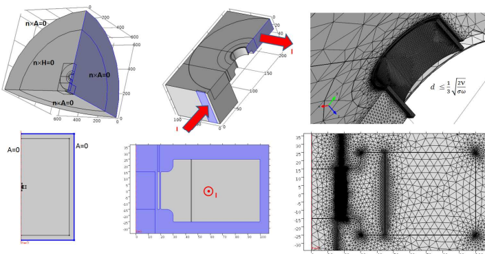
Figure 2. Mesh, Current constraint and Boundary conditions.
