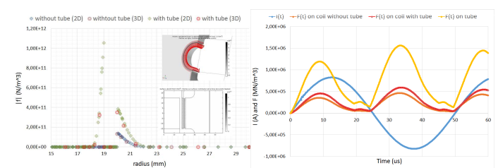
Figure 5. |f|(r) along (\Delta) @ I = 825 \text{ kA} @ \omega/2\pi = 20 \text{ kHz} .
