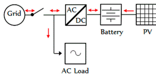
Figure 1. Simplified system power flow schematic.
