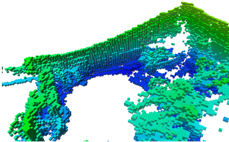
Figure 6: Example of a 3D-grid map, mapping the same place depicted in 2. Each cube is a 5cm side voxel, representing only the occupied space. The color encodes only the height, to help the visualization.
