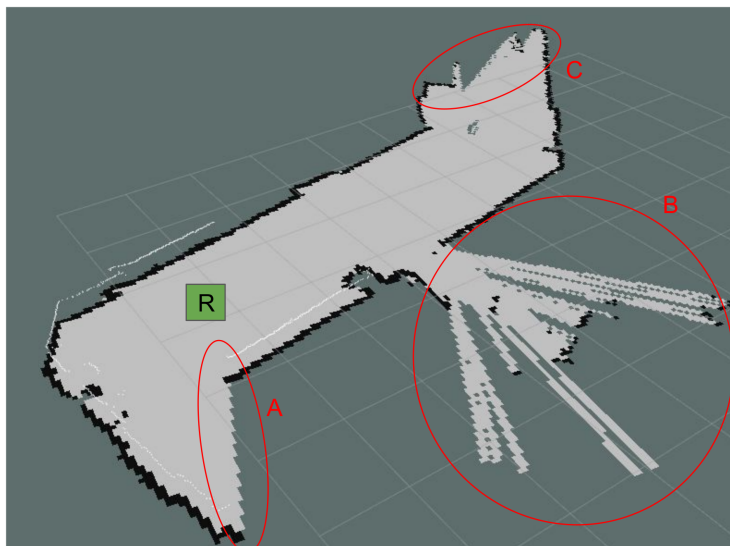
Figure 8: Illustration of the concept of frontier points in an occupancy grid. The current position of the robot is the green square. A, B and C are the main clusters of frontier points
