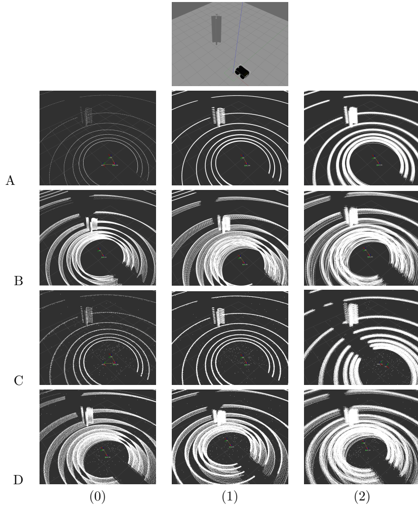
Figure 7: Illustration of the effect of noise on the map, on a toy-case. The noise is applied either on the localization, on the sensor, or on both. Top: the simulation: a husky-robot facing a cross-extruded shape. All the other figures display the point-clouds accumulated for five seconds in a given map frame. The frame is either the perfect localization from the simulation (0), or a noisy localization, where we apply a Gaussian noise to (0). We display two level of noise: (1) and (2). Rows A, B: the Lidar sensor is perfect. Rows C, D: the Lidar sensor is noisy. Rows A, C: the robot is not moving. Rows B, D: the robot is moving. If we focus on the cross-extruded shape, we can see that the higher the noise in the localization and / or on the sensor, the blurrier the shape.
