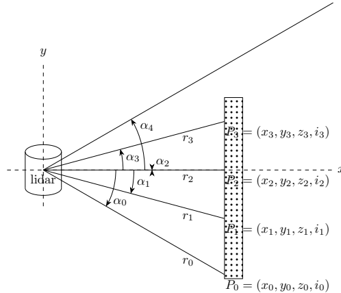
Figure 3: This figure illustrates 3D-Lidar. The light rays are emitted from the Lidar, in known directions (angles \alpha ). When the ray hits an obstacle, the distance of the returned point is computed (distances r ), along with the intensity of the signal i . A point P(x, y, z, i) is added to the point-cloud. Rays that do not return are not in the point-cloud. In this example, although five rays are emitted, the point-cloud contains only four points.
