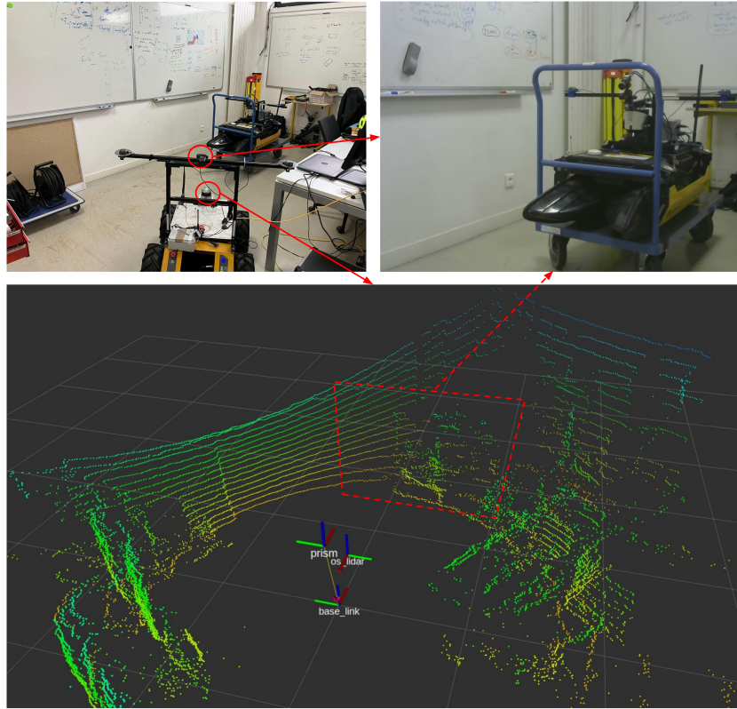
Figure 2: Top-left: external view of the scene. Top-right: image from the camera. Bottom: point-cloud from the Lidar. Top-right and bottom correspond to what the robot "sees". The dashed trapezoid provides an idea of the correspondence between camera and point-cloud. The color in the point-cloud simply encodes the height, for visualization purpose.
