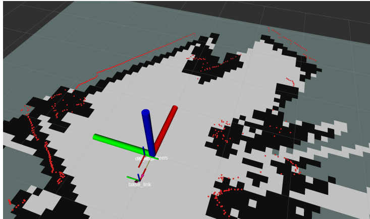
Figure 5: Example of a 2D occupancy grid map, mapping the same place depicted in Figure 2. Black: pixel corresponding to occupied space, light-grey: free space, dark-grey: unknown space.
