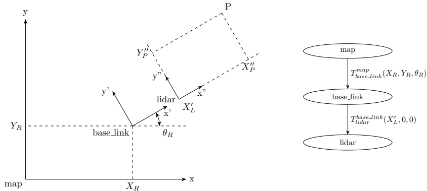
Figure 4: Illustration of the concept of frames in a 2D-example. On the left: different coordinate systems, or frames. The external reference frame is called map , the robot frame is called base_link , and the Lidar frame is called lidar . On the right, the tree structure storing the transformations between frames.
