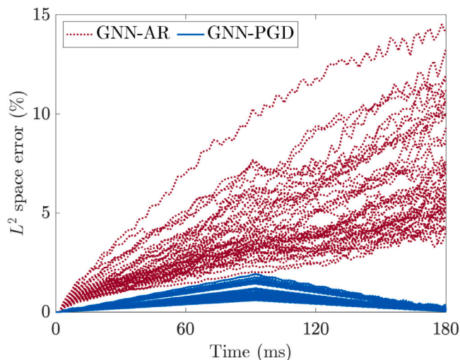
Fig. 19. Comparison of the time evolution of the spatial L^2(\Omega) error between the GNN-AR approach [58,83] and our proposed GNN-PGD approach for the test set \{\Omega_p^{\text{test}}\}_{p=\{1,\dots,50\}} .
