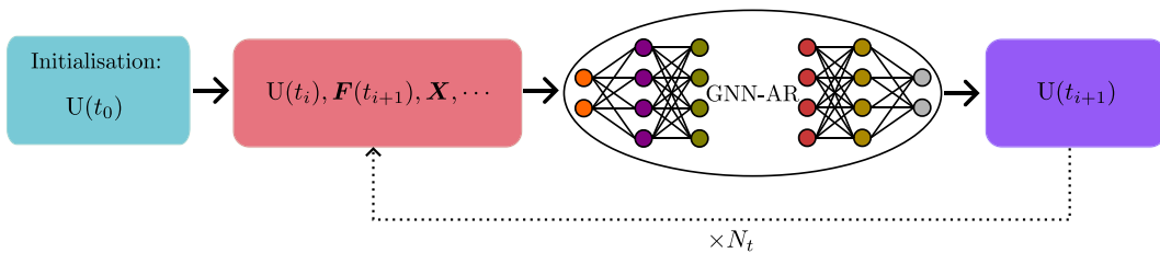
Fig. 18. Illustration of a standard GNN-AR autoregressive approach employed as a benchmark comparison for the proposed GNN-PGD method.
