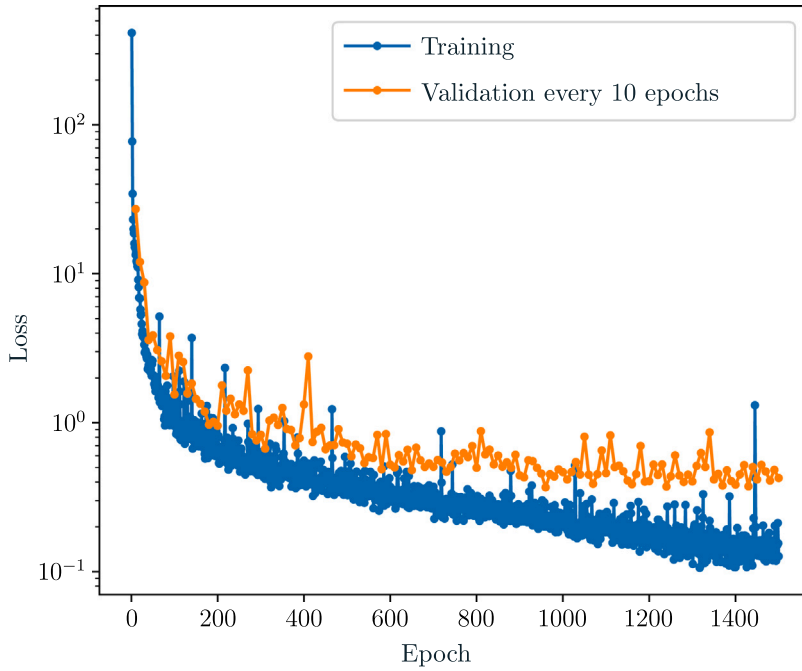
Fig. 10. Evolution of the loss function of the GNN-PGD generator associated with the hyperparameters of Table 4. Every 10 epochs, the loss function is evaluated on the validation database (i.e., the subset not used for training) in order to check that the model is capable of generalizing without over-adjusting. This validation calculation also serves as an early stopping criterion for training.
