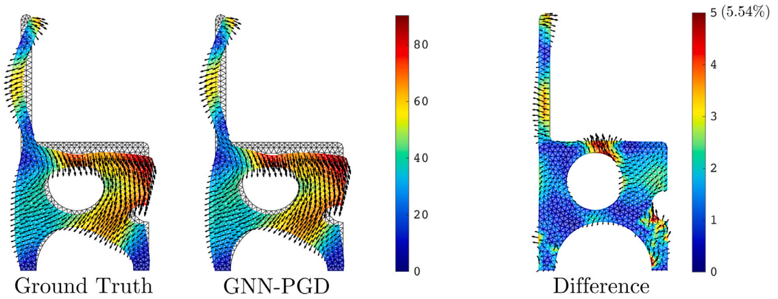
Fig. 15. Example of the third mode predicted by GNN-PGD for seat 44 from the test database, together with the ground truth and error.
