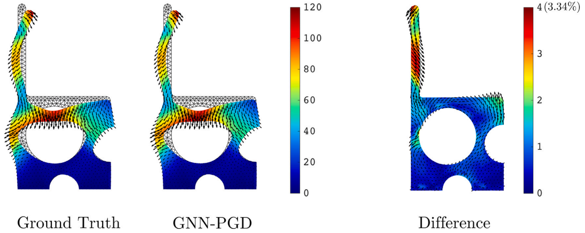
Fig. 14. Example of the third mode predicted by GNN-PGD for seat 23 from the test database, together with the ground truth and error.
