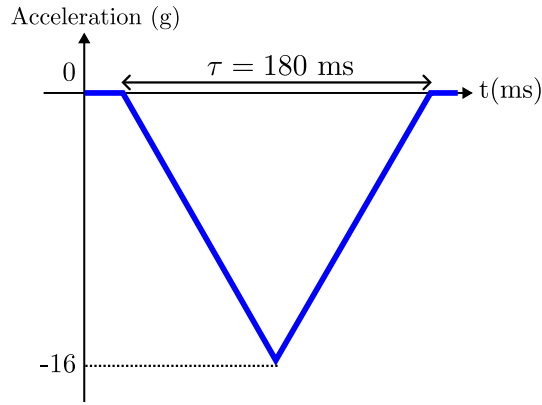
Fig. 6. Loading of interest.
