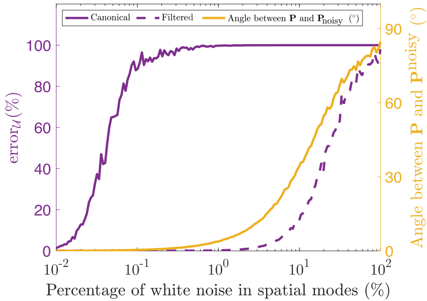
Fig. 5. Effect of the presence of noise in the ROB on the resolution of the projected equation. Three modes have been used to generate the ROB.
