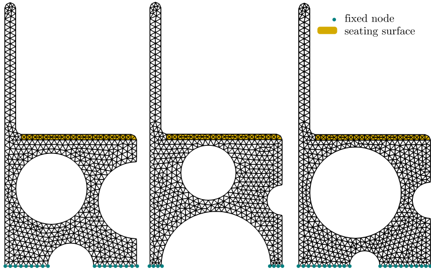
Fig. 8. Example of three seats from the database to illustrate the fixed nodes and seating surface.
