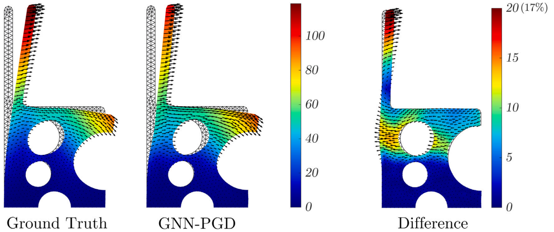
Fig. 21. Mode 1 predicted by GNN-PGD (trained on one hole) on a topology with two holes.
