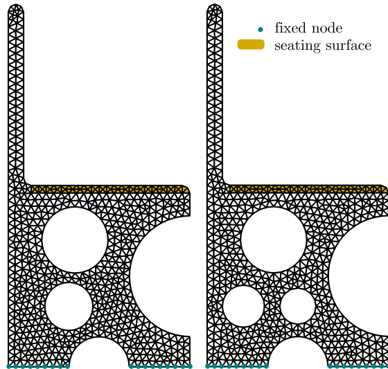
Fig. 20. Example of two seats, exterior to the original database, of very different topologies (i.e., multiple holes).
