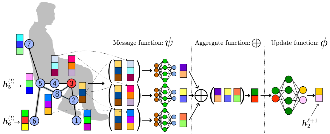
Fig. 4. Illustration of a message passing layer on a three-stage graph applied to another discrete mesh of different size and dimension. The steps for the convolution are identical to that of the example mesh in Fig. 3. Only the Message Transmission step is different since the connectivity of node 3 of this particular graph is different from that of Fig. 3. The aggregate function produces an output state of the same size as that of the example in Fig. 3.
