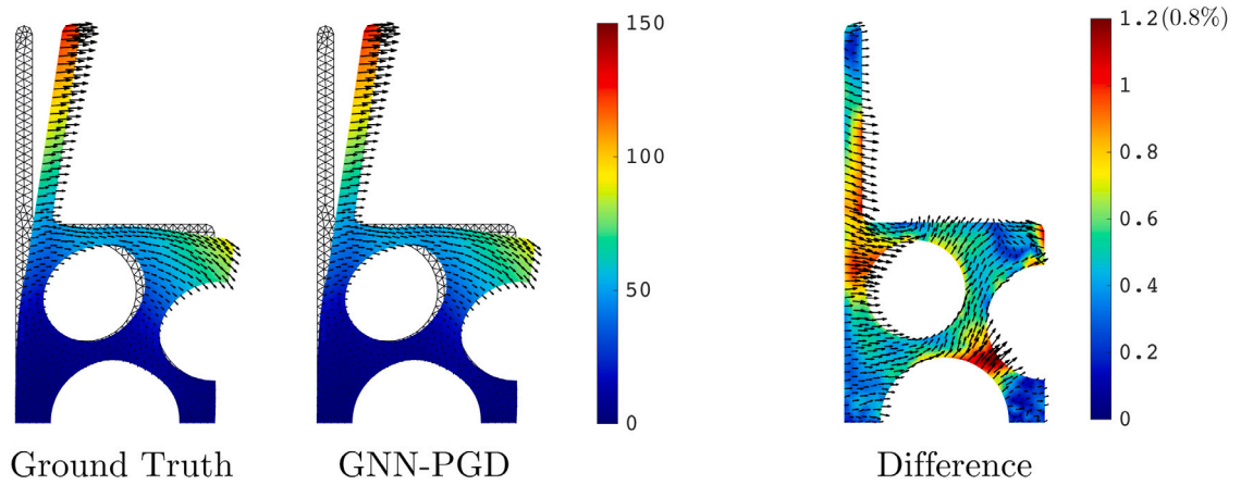
Fig. 12. Example of the first mode predicted by GNN-PGD for seat 1 from the test database, together with the ground truth and error.
