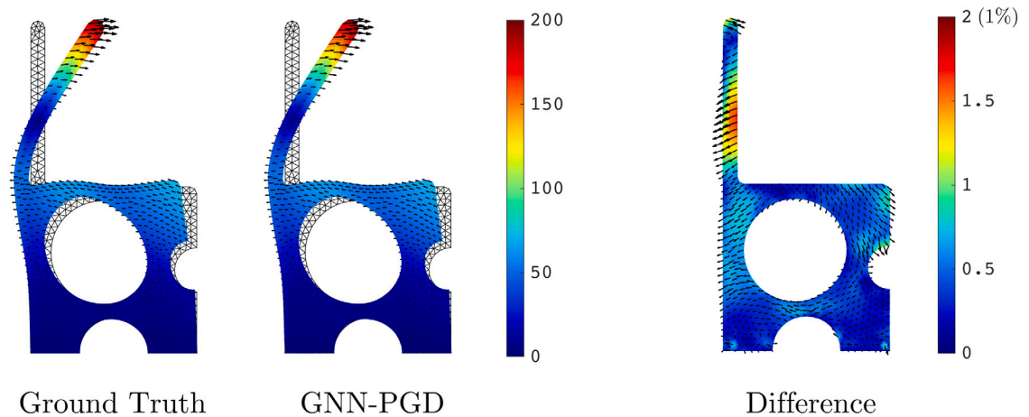
Fig. 13. Example of the second mode predicted by GNN-PGD for seat 10 from the test database, together with the ground truth and error.
