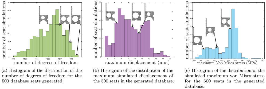
Fig. 9. Statistical analysis of the database used for training, validation, and testing.
