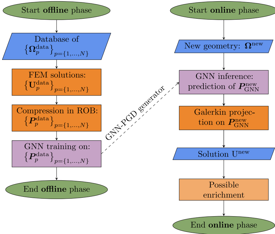
Fig. 2. A flowchart diagram introducing the steps of the proposed GNN-PGD methodology (detailed in Section 3).
