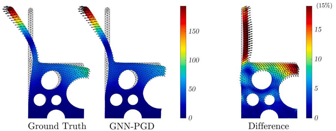
Fig. 22. Mode 2 predicted by GNN-PGD (trained on one hole) on a topology with three holes.
