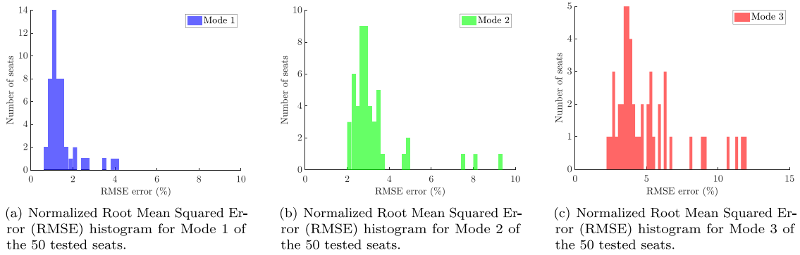
Fig. 11. Results on the modes learned by the GNN-PGD. Errors are calculated between the GNN-PGD spatial modes of displacement and the corresponding labeled PGD spatial modes in the database.
