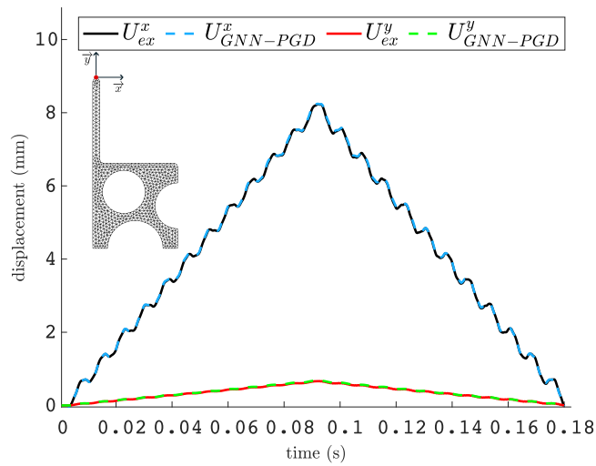
Fig. 17. Displacement of an arbitrary node (whose location is indicated in red) over time, where U_{ex}^x and U_{GNN-PGD}^x are the x -axis displacements of the reference field (FEM) and the field obtained with our proposed methodology, respectively. U_{ex}^y and U_{GNN-PGD}^y denote the y -axis displacements of the reference field (FEM) and the field obtained with our proposed methodology, respectively. (For interpretation of the references to color in this figure legend, the reader is referred to the web version of this article.)
