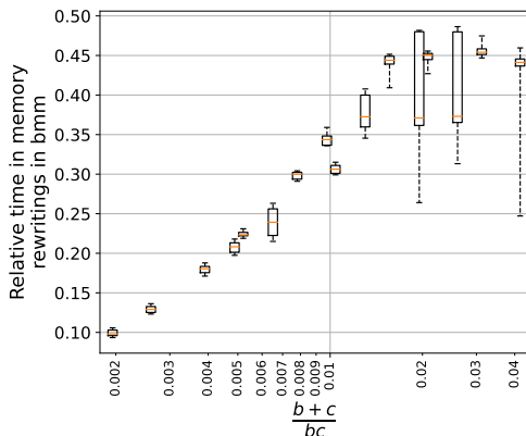
(b) Batch-size-last.
