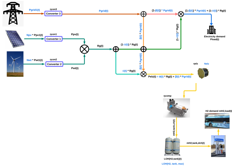
FIG. 1 – Flow Chart of the renewable energy system
