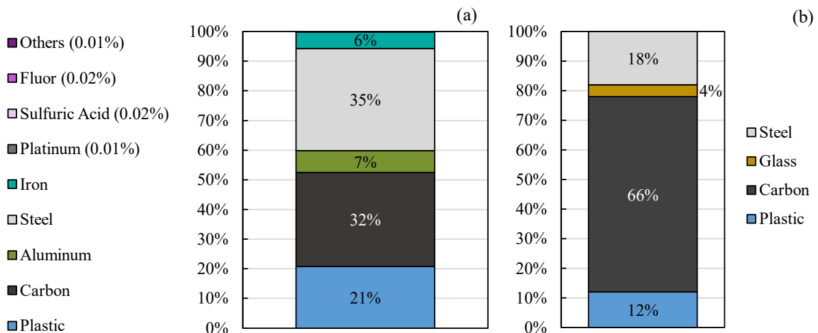
Fig. 2. (a) Mass composition of a PEMFC system and (b) mass composition of a hydrogen tank
