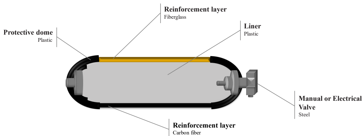
Fig. 3. Composition of a hydrogen tank
