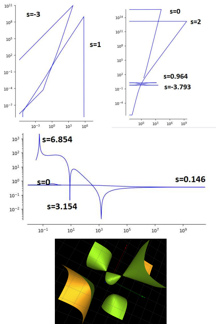
Figure 2. Solutions related to the algebraic surface xyz + x^2 + y^2 + z^2 - x - 2 are indexed in [18]. Up left: the tetrahedral solution 3, up right: solution 21, middle: modulus of solution 42, down: the corresponding algebraic surface. It is a degree 3 del Pezzo surface of the A_1 type.
