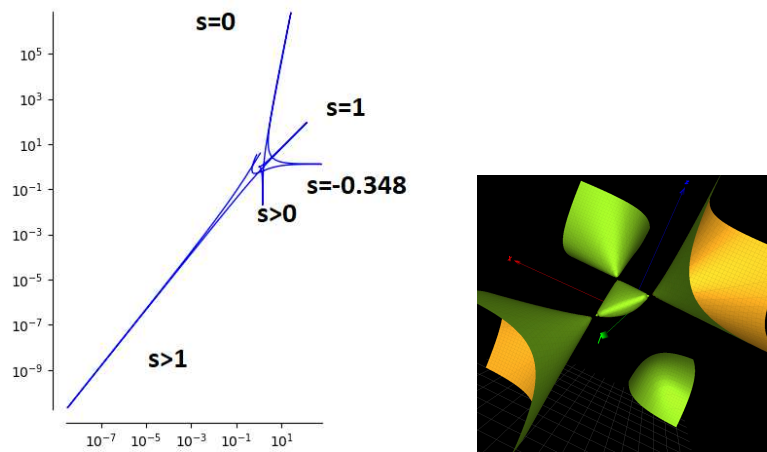
Figure 4. Left: Parametric plot for the modulus of the great dodecahedron solution of P_{VI} (solution 31 of [18, p 157]), the three poles are identified. Right: the corresponding cubic surface is a degree 3 del Pezzo surface of type 3A_1 that is with three isolated singularities).
