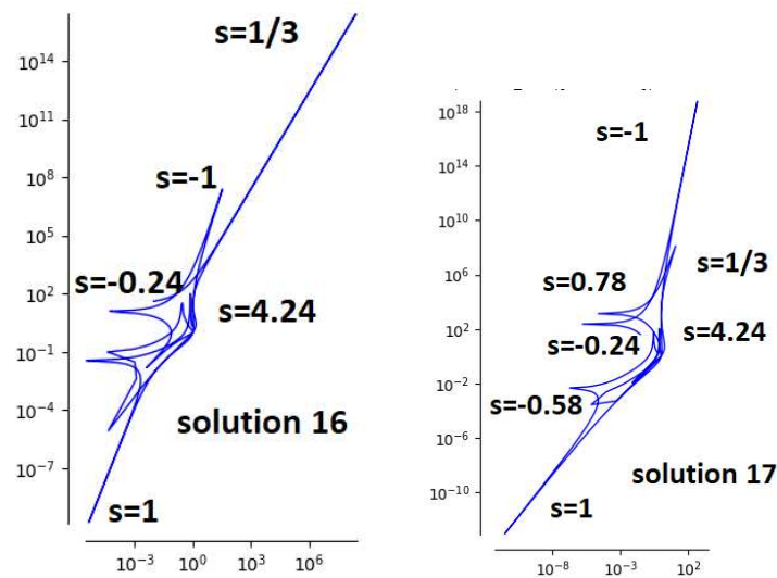
Figure 7. Parametric plots for the modulus of solutions III (the tetrahedral solution), IV (the dihedral solution), solutions 16 and 17 (icosahedral solutions) as first described in [26]. For the later two solutions, we find poles located at irrational values s = -1, 1/3, 2 \pm \sqrt{5} and \pm 1/\sqrt{3} .
