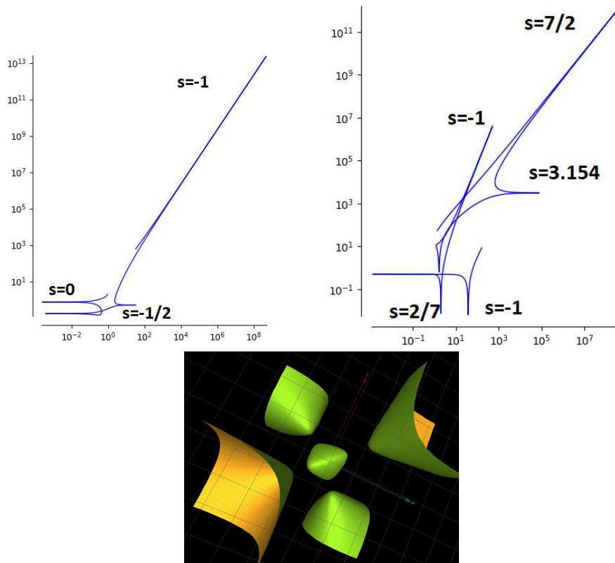
Figure 3. Solutions related to the algebraic surface xyz + x^2 + y^2 + z^2 - 3 = 0 are indexed in [18]. Up left: the modulus of the octahedral solution 20, up right: the modulus of solution 45, down: the corresponding algebraic surface.
