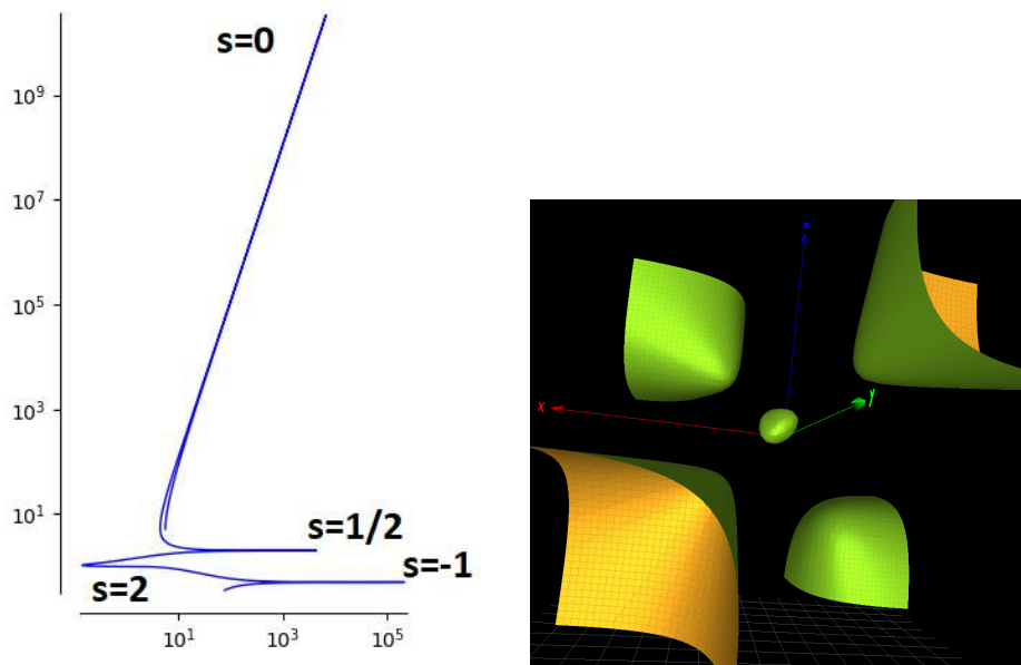
Figure 1. Left: Parametric plot for the modulus of Klein solution of P_{VI} (solution 8 of ([18] p 157)), the discontinuities of the plot correspond to the four poles. Right: the corresponding cubic surface xyz + x^2 + y^2 + z^2 - x - y - z = 0 .
