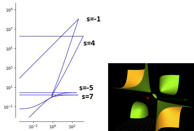
Figure 6. Left: Parametric plot of an icosahedral solution of P_{VI} (solution 7 of [18, p 157]), the discontinuities of the plot correspond to the poles. Right: the corresponding cubic surface.
