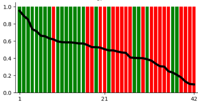
gpt3.5
