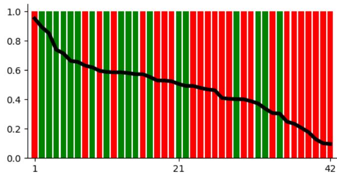
mistral
