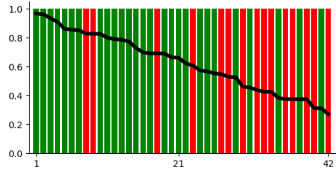
mistral
