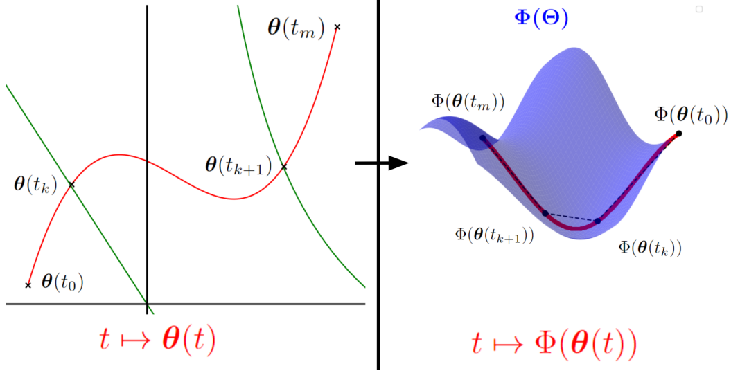
Figure 1: Illustration of the proof of Theorem 3.1, see the end of Section 3 for an explanation.
