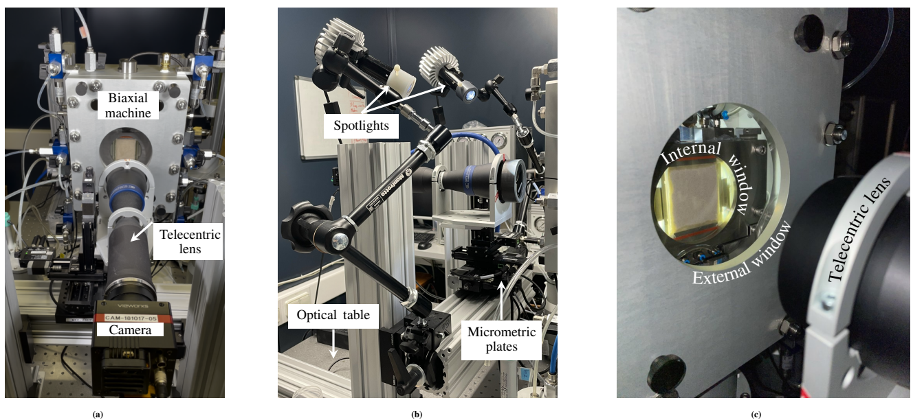
Figure 2 (a) Biaxial machine endowed with its optical system, (b) photograph showing the additional elements to the acquisition setup, (c) close up on the biaxial machine highlighting the internal/external windows from one-side view.
