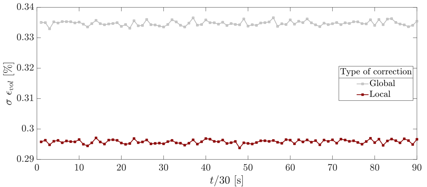
Figure 12 Evolution of the standard deviation value of the volumetric strain derived from DIC calculation with a Tikhonov regularization of 15 pixels and mesh size of 5 pixels and tested under two types of gray level correction, over an acquisition period of 3s.
