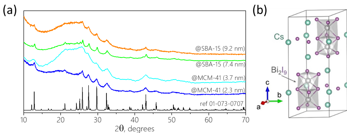
Figure 2. a) XRD pattern of \text{Cs}_3\text{Bi}_2\text{I}_9 encapsulated in various mesoporous matrices (14.5 mass. %). Reference (black line): ICDD 01-073-0707; b) Schematic illustration of a unit cell of \text{Cs}_3\text{Bi}_2\text{I}_9 with a 0D dimer structure.
