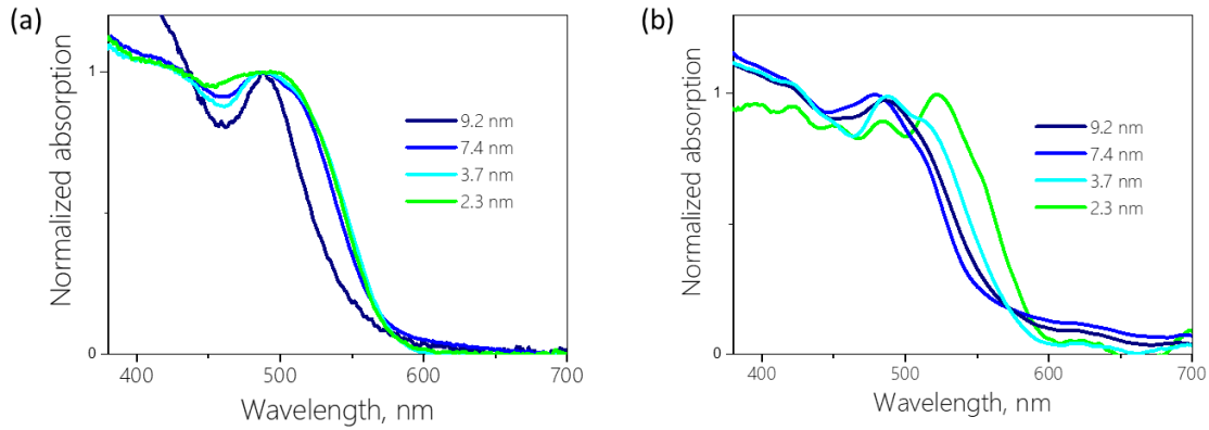
Figure 3. Absorption spectra of \text{Cs}_3\text{Bi}_2\text{I}_9 (14.5 mass. %, left, and 7.3 mass.%, right) encapsulated in various mesoporous matrices
