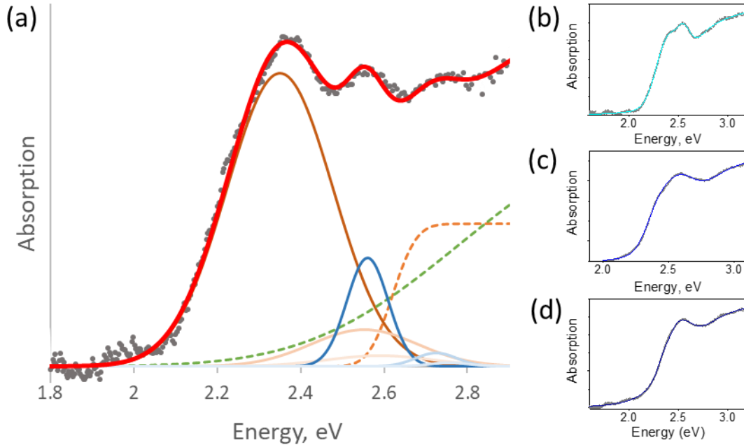
Figure 4. a) Absorption spectrum of Cs_3Bi_2I_9@MCM-41 (2.3 nm, 7.3 mass. %) (grey dots) fitted with a double Elliott curve (red). The constituents of the fit are highlighted: the continuum curve (dotted green), as well as two series of excitonic peaks (shades of orange and shades of blue); Absorption spectra with Elliott fit of: Cs_3Bi_2I_9 encapsulated in MCM-41 (3.7 nm, 7.3 mass. %) (b), SBA-15 (7.4 nm, 7.3 mass. %) (c), and SBA-15 (9.2 nm, 7.3 mass. %) (d).
