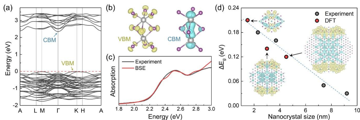
Figure 5. (a) Band structure of \text{Cs}_3\text{Bi}_2\text{I}_9 . (b) Charge density distributions of VBM and CBM within a single \text{Bi}_2\text{X}_9 dioctahedron. Color code: grey for Bi and purple for I. (c) Optical absorption spectrum of \text{Cs}_3\text{Bi}_2\text{I}_9 from experiment ( \text{Cs}_3\text{Bi}_2\text{I}_9 @SBA-15, 9.2 nm, 7.3 mass. %) and calculation (bulk model). The computational curve is shifted to match the excitonic peak. (d) Bandgap changes between the confined systems with different sizes and the bulk \text{Cs}_3\text{Bi}_2\text{I}_9 . ( E_g^{\text{confined}} - E_g^{\text{bulk}} ). The top view of the computational models and the relevant charge density distributions of VBM (yellow) and CBM (blue) are plotted.
