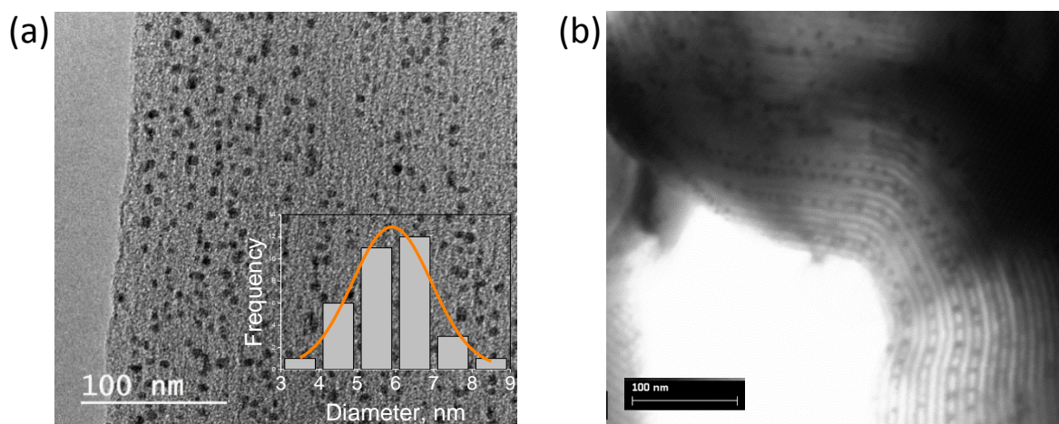
Figure 1. TEM (a) and STEM (b) images of \text{MA}_3\text{Bi}_2\text{I}_9@\text{SBA-15} (7.4 nm pore size, 14.5 mass.%), inset shows the size histogram of the NCs in the pores.
