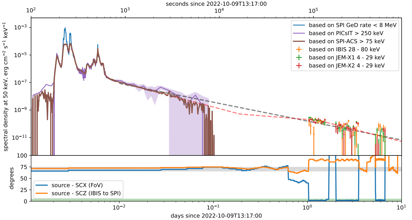
Fig. 3. GRB 221009A prompt emission and afterglow lightcurve (top). All count rates are converted to a spectral energy density at 50 keV assuming powerlaw spectrum with a slope of -2 . This spectrum is applicable for the afterglow, but implies that the prompt lightcurve in this plot is only indicative. Note: the “all-sky” observations are also available between 0.1 and 1 days after the event, but the uncertainty due to the remaining background variations does not allow for a measurement to be made within this time range. The gray dashed line represents a fit with a single powerlaw, acceptable given the response uncertainties. Red dashed line represent best fit model, consisting of powerlaw segments with two breaks. For details about the fitting see explanations in the text. GRB 221009A position relative to INTEGRAL spacecraft orientation, relevant for changes of the instrument response throughout the emission phases (bottom). The gray band indicates the range of orientations when the response changes by no more than 30%. The green band represents approximate FoV of INTEGRAL instruments.
