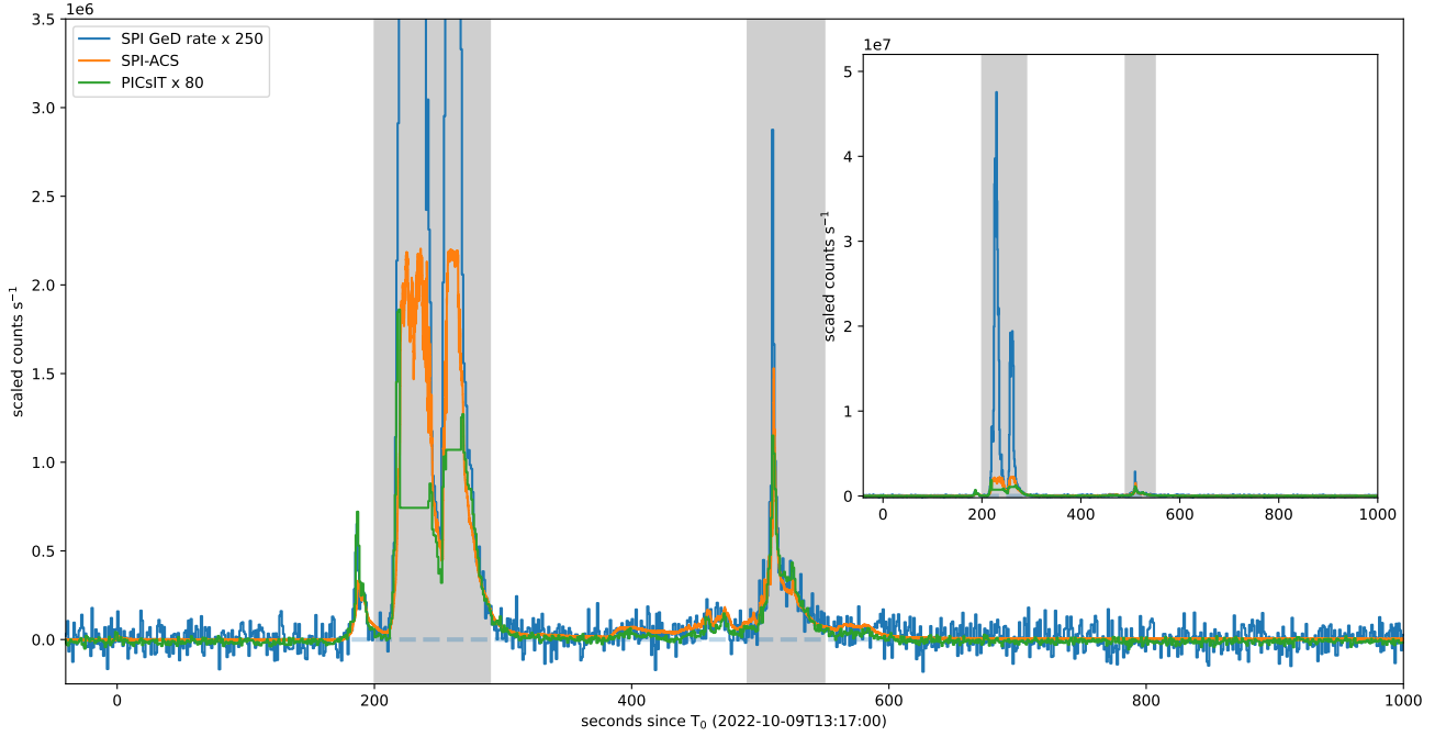
Fig. 1. GRB 221009A prompt emission light curves (background-subtracted) as recorded by INTEGRAL instruments: SPI, SPI-ACS, and IBIS/PICsIT. All rates except for SPI-ACS are normalized to match the SPI-ACS rate. The SPI-ACS rate is affected by saturation for count rates above about 1.8 \times 10^6 counts s^{-1} and for PICsIT by the INTEGRAL buffer limit. Inset shows the different count rate range (in the same time range), highlighting combined SPI (Germanium detectors) rate (only moderately affected by dead-time), giving some insight on the true intensity of the primary emission episode comparing to the rest of the signal. Vertical dashed lines represent boundaries of the INTEGRAL pointings (see details in Sect. 2). Gray shaded regions represent emission episodes used for estimating fluence.
