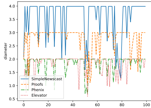
Fig. 12: Diameter computed with a hub-targeted attack, for each algorithm, every 10 cycles
