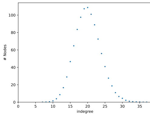
Fig. 29: In-degree distribution of the network, after the run of the PROOFS algorithm for 1000 cycles.
