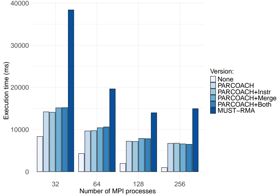
Fig. 8: Execution time of MiniVite with a problem size of 1,280,000, depending on the number of processes and the approach used.
