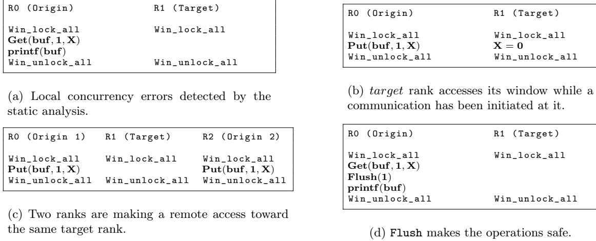
Fig. 7: Examples of the different types of data races. X represents the window of R1.
