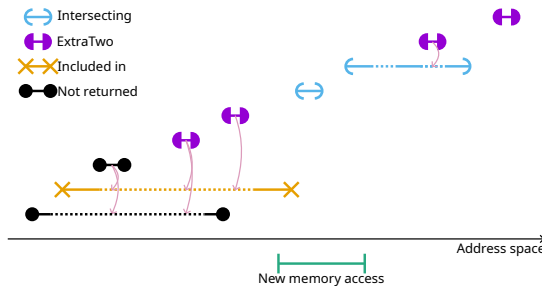
Fig. 5: Determining which intervals are intersecting with the new access.
