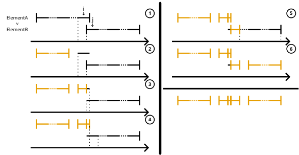
Fig. 6: Fragmentation process of two intersecting intervals.
