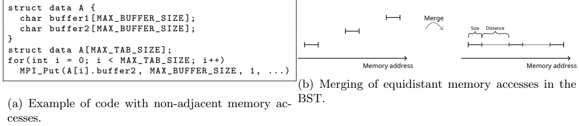
Fig. 3: Example of a code making non-adjacent memory accesses and how the latter should be represented in the BST.
