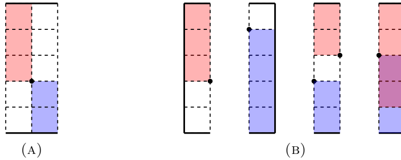
FIGURE 4. Figure A): In each fiber, there is exactly one red or blue cell induced by each point of the permutation, as stated by (7.1). Figure B): From left to right, we show the cases in R), L), I0) and I1), respectively.
