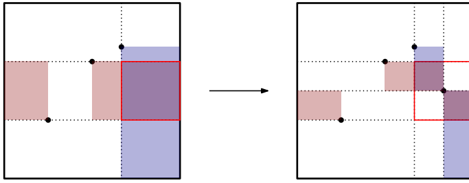
FIGURE 6. Relative order of \pi_n(n) , \pi_n^{-1}(\ell) and \pi_n^{-1}(\ell - 1) in case 1). The blue cells are cells with \Delta D_{n+1} = 1 and the red cells are cells with \Delta D'_{n+1} = 1 .
