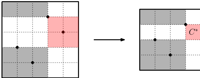
FIGURE 5. Permutation \pi_3 = (213) (to the right) induced from \pi_4 = (2143) (to the left) when taking out \pi_4(4) = 3 . We keep track of the increment behavior of the red cell during the induction.
