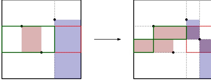
FIGURE 7. Relative order of \pi_n(n) , \pi_n^{-1}(\ell) and \pi_n^{-1}(\ell - 1) in case 2). The blue cells are cells with \Delta D_{n+1} = 1 and the red cells are cells with \Delta D'_{n+1} = 1 .
