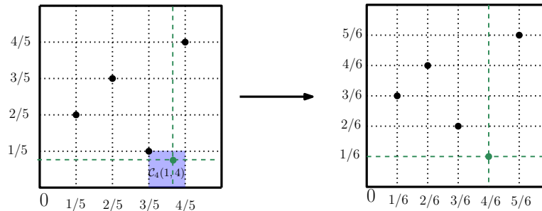
FIGURE 1. Graphical representation of \pi_4 = (2314) to the left. We colored in light blue the cell \mathcal{C}_4(1, 4) . We represent to the right-side the resulting permutation \pi_5 = (34215) when u \in \mathcal{C}_4(1, 4) . We present the point u and vertical and horizontal lines crossing it in green in order to visually see the transformation.
