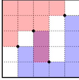
FIGURE 3. Coloring of the graphical representation associated to \pi_4 = (2314) .
