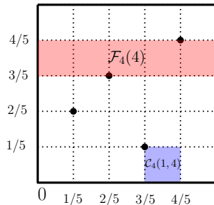
FIGURE 2. Graphical representation of \pi_4 = (2314) to the left. We colored in light blue the cell \mathcal{C}_4(1, 4) and in light red the cells belonging to the fiber \mathcal{F}_4(4) .
