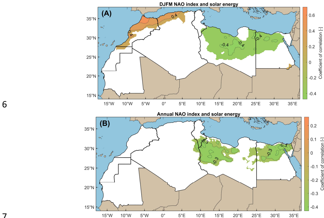
8 Fig. 2. Spearman correlation between NAO index and Solar resources in the North Africa 9 region. Please note the different scales on the color bar. Only significant correlations ( p 10 < 0.05 ) are shown.
