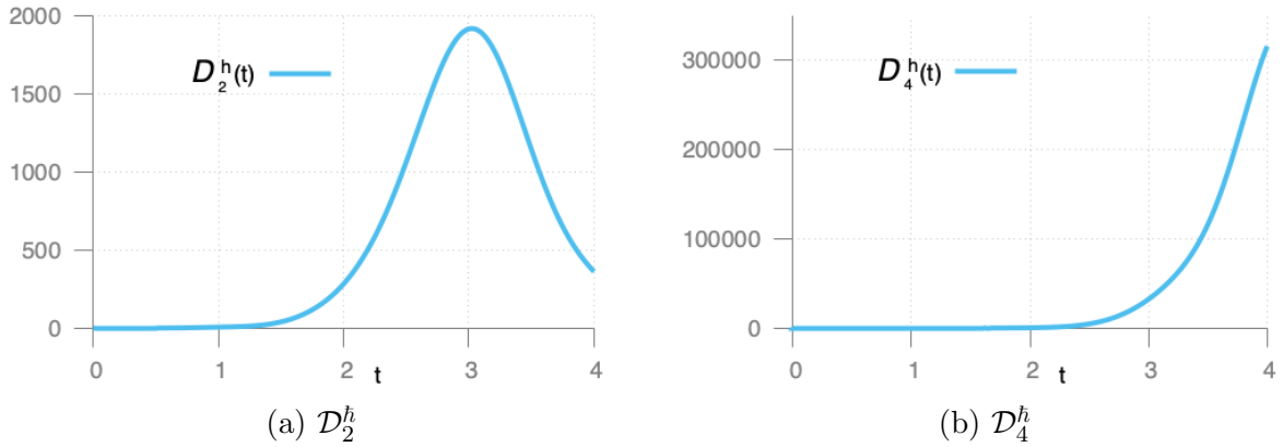
FIGURE 4.9. Quantum tunneling : Time evolution of the quantities D_2^h and D_4^h for h = 1 .
