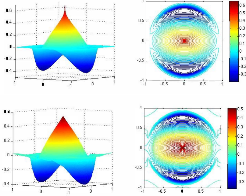
FIGURE 4.1. Solution of Bourgain-Brezis problem with 2D data in (4.11). Helmholtz solution, \mathbf{u}_{\text{Hel}} (top), vs. two-step solution, \mathbf{u}_{\text{2step}} (bottom).
