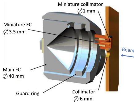
Figure 6. Miniature Faraday cup (FC) for online beam monitoring.
