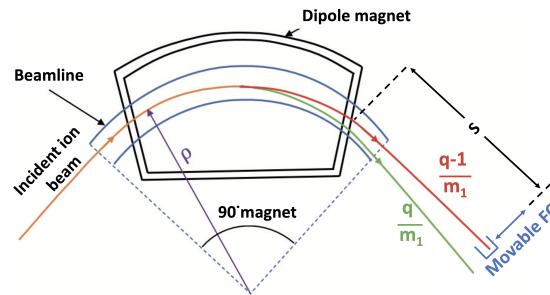
Figure 7. Movable FC to continuously measure the current of the adjacent ( q-1 ) ion beam while the beam of interest ( q ) is transported further in the beam line.
