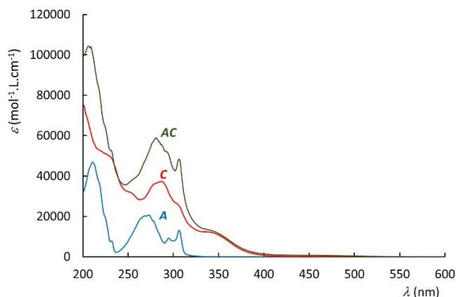
Figure 4 UV-visible spectra in acetonitrile, for A , C , and AC .
