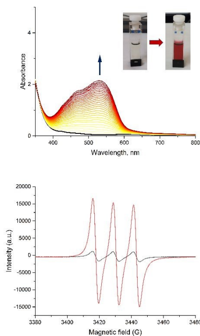
Figure 8 Griess-test showing the appearance of a pink dye with \lambda_{\text{max}} around 540 nm (top) and triplet signal from Fe-MGD-NO formed in EPR experiment (bottom) for AC at room temperature at \lambda = 365 \text{ nm} irradiation.
