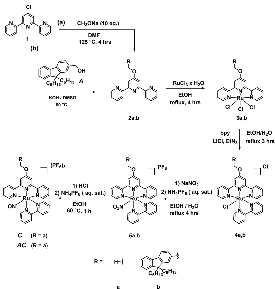
Scheme 3 Synthesis of C and AC .
