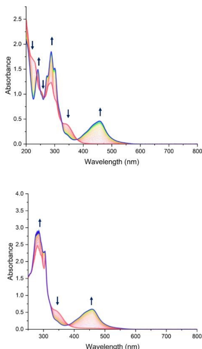
Figure 7 Evolution of UV-Vis spectra of C (top) and AC (bottom) in acetonitrile under 2 hours of irradiation at \lambda = 365 nm, with starting complex C in red and photoproduct in blue.
