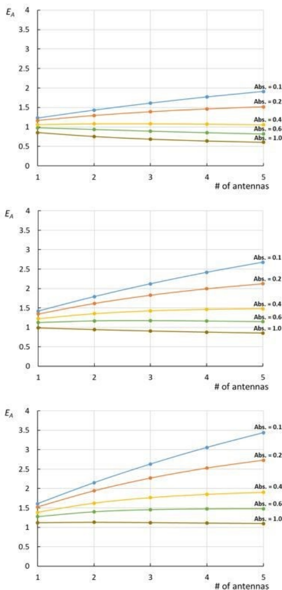
Figure 1 Relative efficiency E_A (equation 11) expressed at various \Phi_A \cdot E_{FRET} values [0.3 (top), 0.5 (middle), and 0.7 (bottom)] for complexes bearing 1 to 5 antennas. On each graph, the curves are drawn at various of absorbance ranging from Abs. = 0.1 to 1.0, with the assumption that \varepsilon_A = \varepsilon_C .
