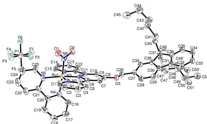
Figure 3 Asymmetric unit of [\text{FCH}_2\text{OTRu}(\text{NO}_2)](\text{PF}_6) with atom labeling scheme. Hydrogens are omitted for clarity.
