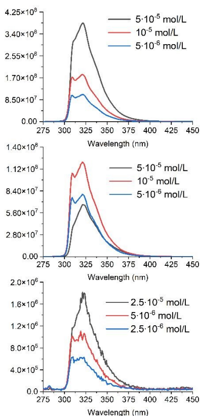
Figure 6 Graphs of fluorescence intensities for A (top), A+C (middle) and AC (bottom) in acetonitrile, recorded at 3 different concentrations.
