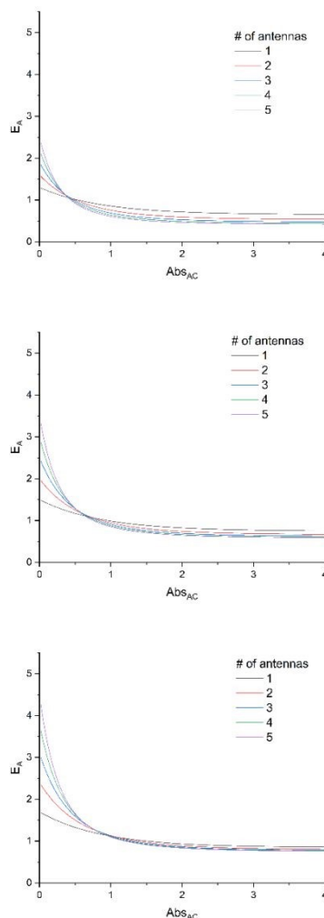
Figure 2 E_A expressed at various \Phi_A \cdot E_{FRET} values [0.3 (top), 0.5 (middle), and 0.7 (bottom)] for complexes bearing 1 to 5 antennas, according to equation (11), with the assumption that \varepsilon_A = \varepsilon_C .
