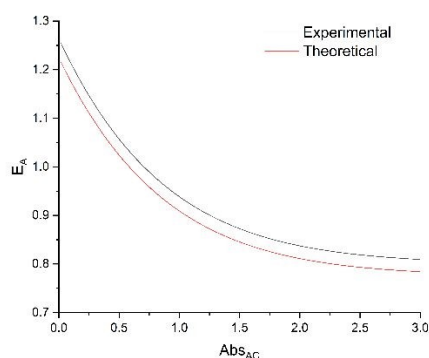
Figure 9 Relative efficiency E_A (equation 11) calculated from NO release data ( \Phi_C and \Phi_{AC} ) as the “experimental” curve, compared with the values predicted from the antenna data ( \Phi_A = 0,387 ) as the “theoretical” curve..
