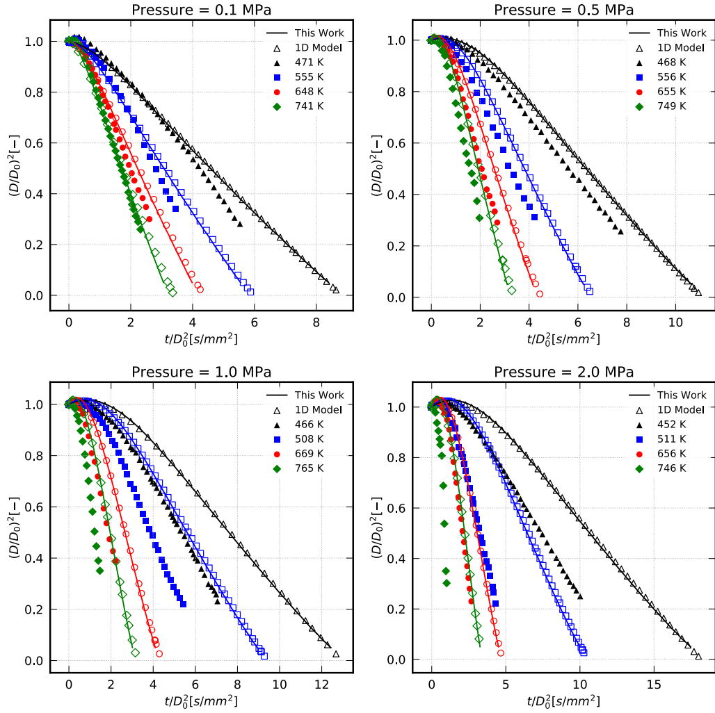
Figure 8: Square diameter decay at different pressure and temperature for the microgravity evaporation of n-heptane. Comparison with experiments from Nomura et al. [3] (filled markers), and with the spherically-symmetric 1D model by Cuoci et al. [12] (empty markers) ( http://basilisk.fr/sandbox/ecipriano/run/microgravity.c ).
