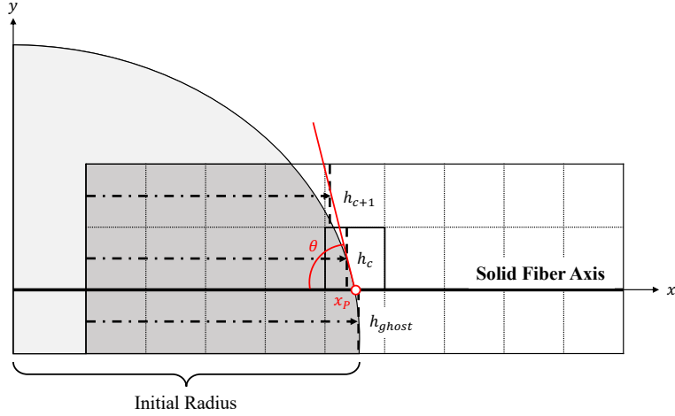
Figure 2: Schematic representation of the height function boundary conditions, where the black line represents the solid fiber surface, the white point is the pinning point \mathbf{x}_p , while \theta is the contact angle.
