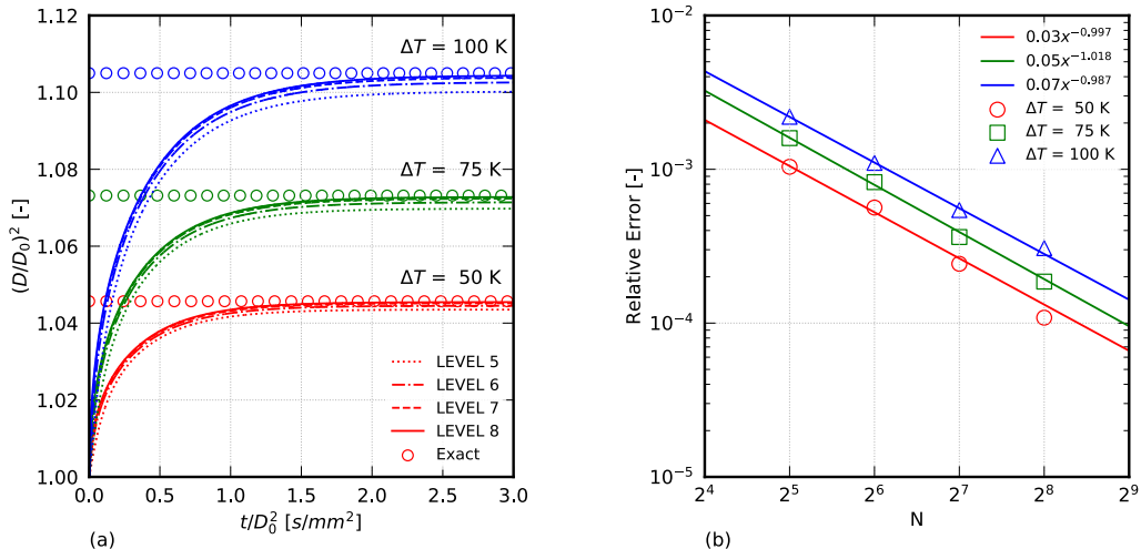
Figure 6: Evolution of the normalized square diameter for the droplet expansion problem at different \Delta T between the droplet and the environment (a); convergence rate for the droplet expansion problem (b) ( http://basilisk.fr/sandbox/ecipriano/run/expansion.c ).
