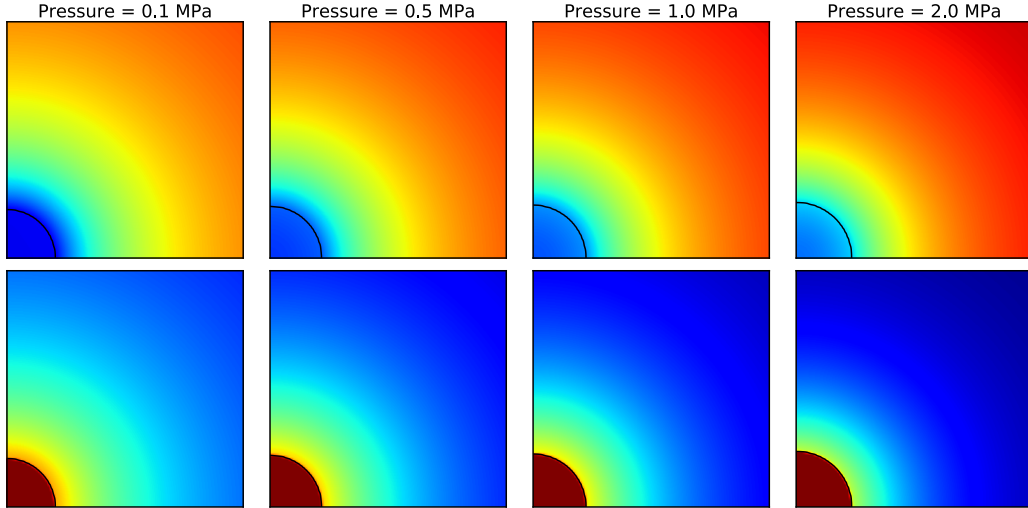
Figure 7: Maps of temperature (top) and n-heptane mass fraction (bottom) at different ambient pressures in microgravity conditions at T \approx 750 K and time 0.6 s ( http://basilisk.fr/sandbox/ecipriano/run/microgravity.c ).
