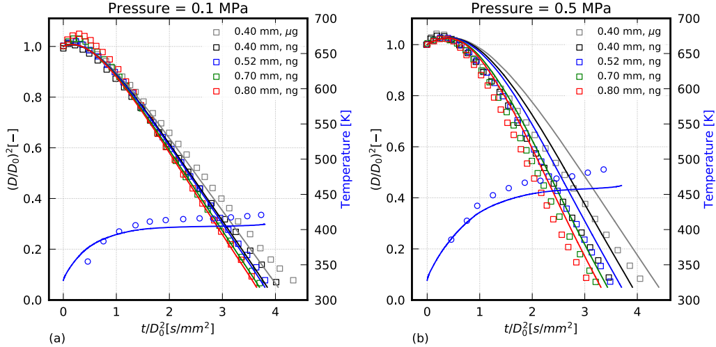
Figure 11: Normalized squared diameter and temperature profile for the n-decane evaporation in normal gravity conditions (ng) and in microgravity ( \mu g ). Comparison with experiments by Murakami et al. [5] ( http://basilisk.fr/sandbox/ecipriano/run/normalgravity.c ).
