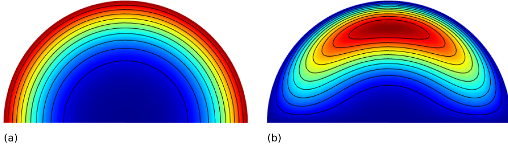
Figure 5: Maps of the temperature (a) and velocity divergence (b) inside the liquid droplet, for the thermal expansion test case at time 0.1 s. The divergence field embeds the AXI metrics.
