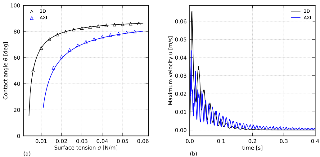
Figure 4: Equilibrium contact angles, where the lines are the analytic solutions, while the markers are the numerical results (a); relaxation of the maximum velocity for the 2D and AXI cases (b) ( http://basilisk.fr/sandbox/ecipriano/test/pinning.c ).
