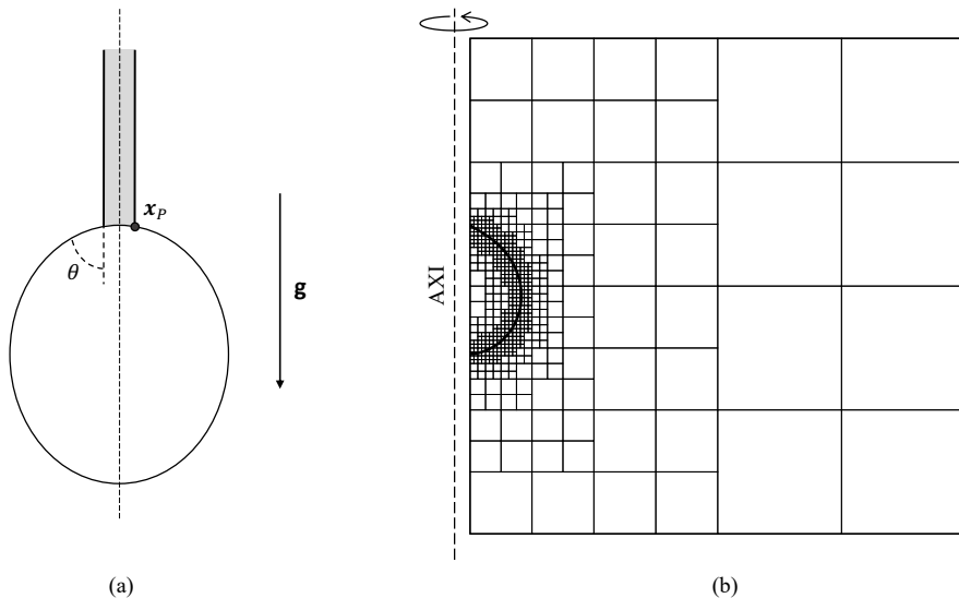
Figure 1: Simulation setup for suspended droplets in normal gravity conditions. Schematic representation of the droplet suspended on a solid fiber, with contact angle \theta , pinning point \mathbf{x}_p , and gravity \mathbf{g} (a); simulation setup for the axial-symmetric suspended droplet configuration, using an adaptive grid (b).
