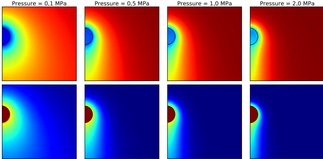
Figure 9: Maps of temperature (top) and n-heptane mass fraction (bottom) at different ambient pressures in normal gravity conditions at time 0.6 s ( http://basilisk.fr/sandbox/ecipriano/run/normalgravity.c ).
