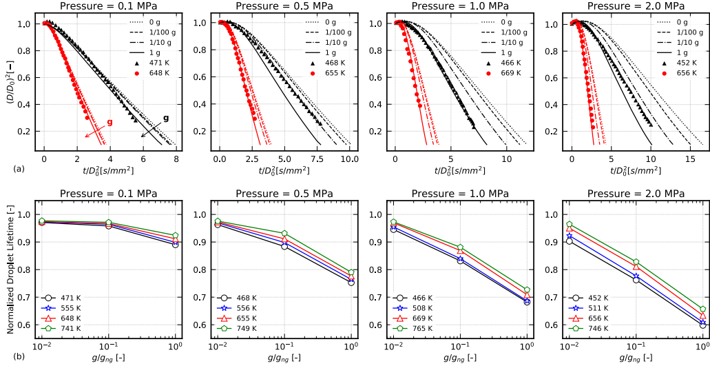
Figure 10: Squared diameter decay at different pressure and temperature, and at 4 different gravitational acceleration values. The triangles are experiments from Nomura et al. [3] (a); Normalized total evaporation times (b) ( http://basilisk.fr/sandbox/ecipriano/run/normalgravity.c ).
