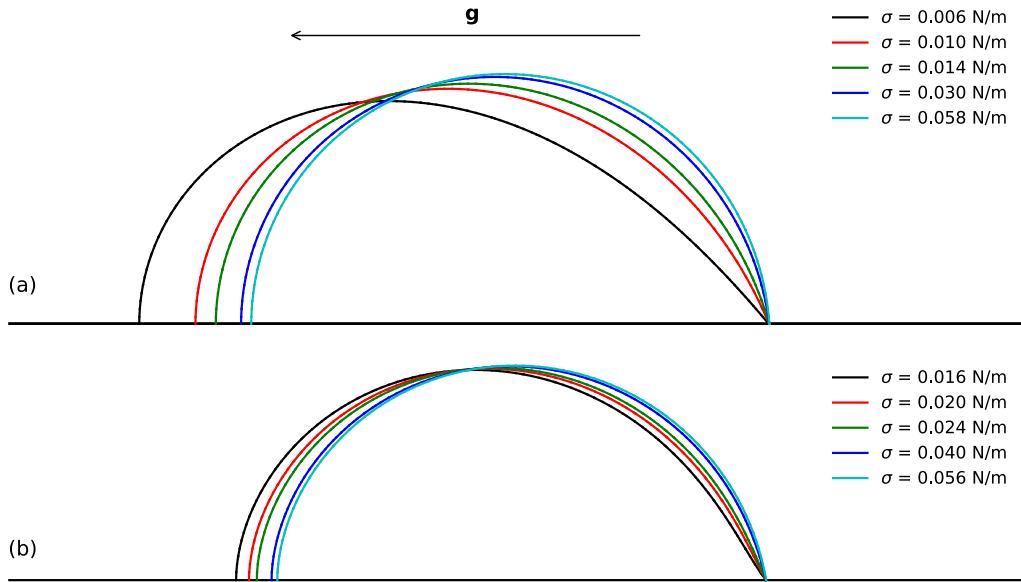
Figure 3: Equilibrium shape for the 2D (a) and AXI (b) suspended droplets, with gravity pointing leftward with respect to the figures.
