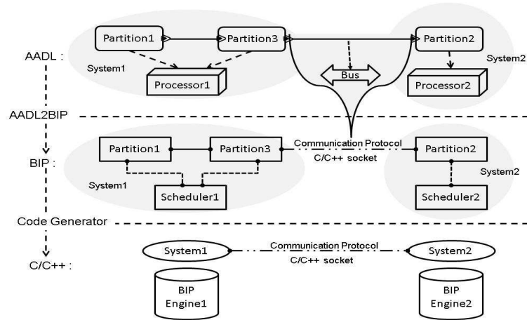
Fig. 4. Deployment
