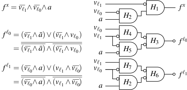
Fig. 19: Encoding of functions f^x , f^{\ell_0} , f^{\ell_1} as And-Inverter Graphs based on Irredundant Sums-of-Products.
