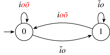
(b) Strategy yielded by the automaton of Figure 29a for the formula G((i \wedge \delta) \vee \bar{i}) \leftrightarrow GF(o)
