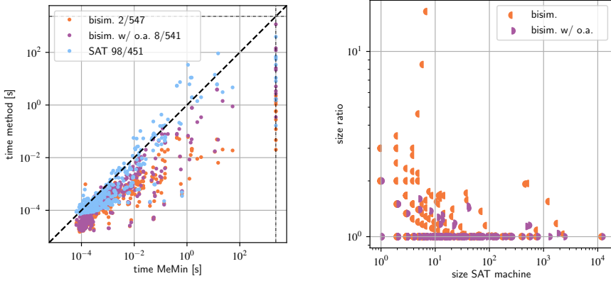
(a) Total runtime for instances derived from SYNTCOMP. (b) Size ratios for instances derived from SYNTCOMP.
