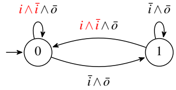
(b) Strategy yielded by the automaton of Figure 30a for the formula (\text{GF}(i) \leftrightarrow \text{GF}(\bar{i} \wedge o))
