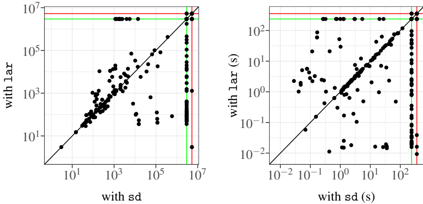
(a) Comparison of the size of the parity games obtained with the sd and 1ar configurations (b) Minimal total time used by ltlstxt with sd and 1ar to produce a game
