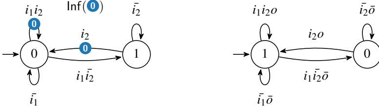
(a) Büchi automaton associated to GF(i_1) \wedge GF(i_2)
