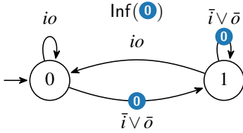
(a) Büchi automaton associated with GF((i \wedge \delta) \vee \bar{i})
