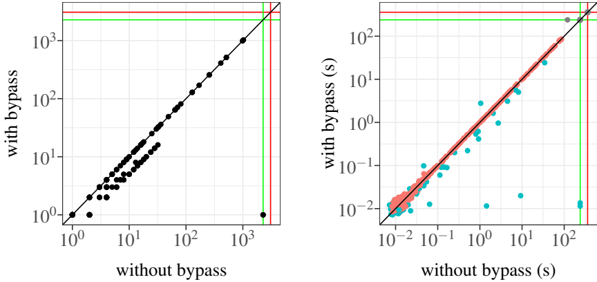
(a) Number of states with and without bypass on the set of cases that can be bypassed
