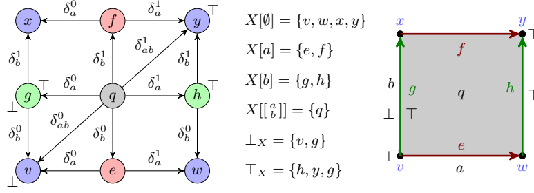
Fig. 5: A two-dimensional HDA X on \Sigma = \{a, b\} , see Ex. 7.
