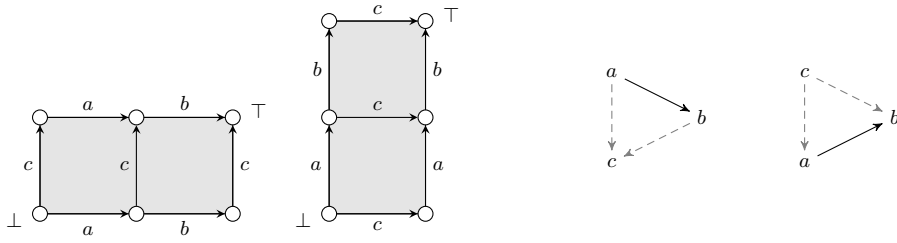
Fig. 7: HDA X which accepts language L of Ex. 28 and the two generating ipomsets in L .
