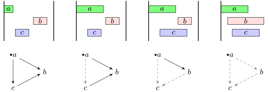
Fig. 2: Activity intervals of events (top) and corresponding ipomsets (bottom), cf. Ex. 1. Full arrows indicate precedence order; dashed arrows indicate event order; bullets indicate interfaces.
