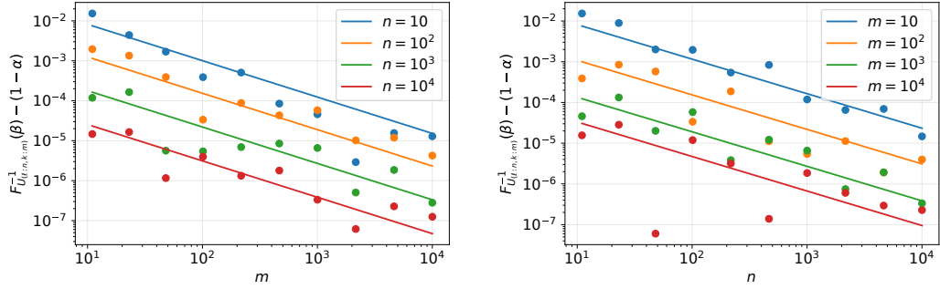
FIG 14. QQC: log-log plot of \Delta q_\beta as a function of m (left) or n (right). Lines show the approximation \log \Delta q_\beta \approx \log(c_2) - \gamma_2 \log(m) - \delta_2 \log(n) with c_2, \gamma_2, \delta_2 given by Table 1.
