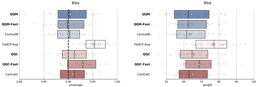
FIG 8. Coverage (left) and average length (right) of prediction intervals for 50 random learning-calibration-test splits of the bike data set. The miscoverage is \alpha = 0.1 , \beta = 0.2 , and the calibration set is split into m = 40 disjoint subsets of equal size n = 10 . See the beginning of Section 6.2.2 for details.
