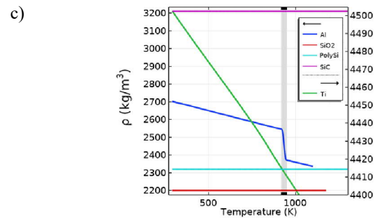
Figure 9. The evolution of a) Heat capacity, b) Thermal conductivity and c) Density as a function of temperature for Al, SiO 2 , Ti, SiC, and poly-Si [9]
