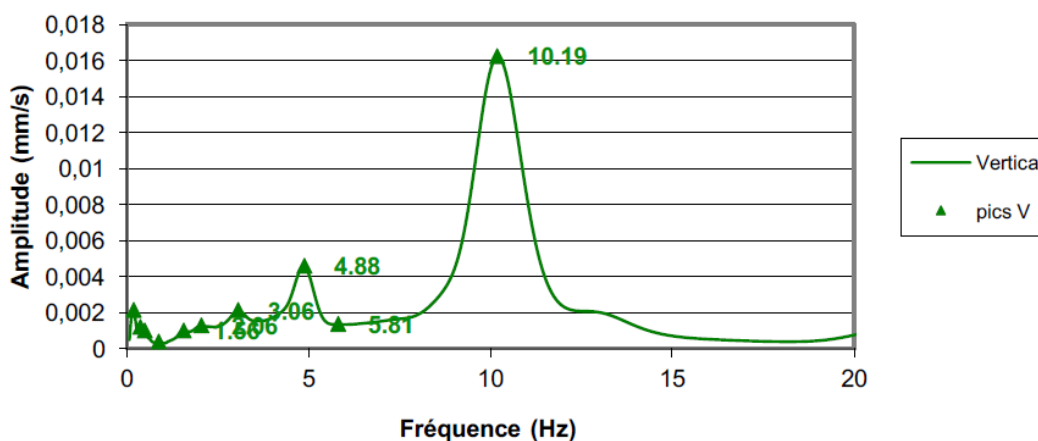
Figure 14: Natural frequency measured with the ‘velocimeter’
