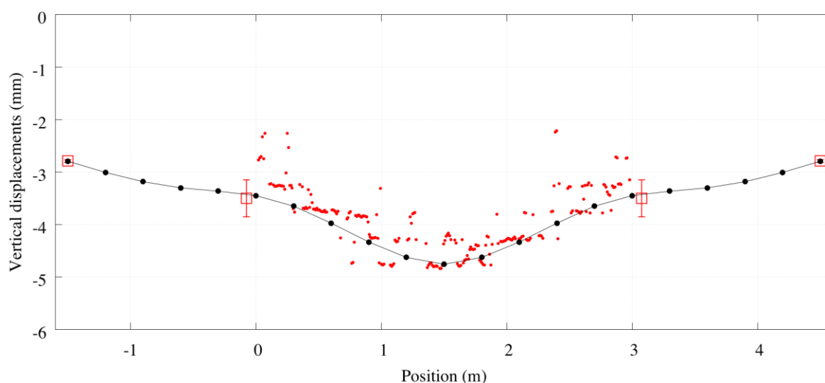
Figure 13: Vertical displacements along an upper chord of the structure: (black line) prediction of the initial model, (red dots) DIC measurements, (square symbols) comparator measurements.
