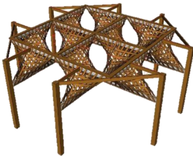
Figure 1: A 3D view of the structure model
