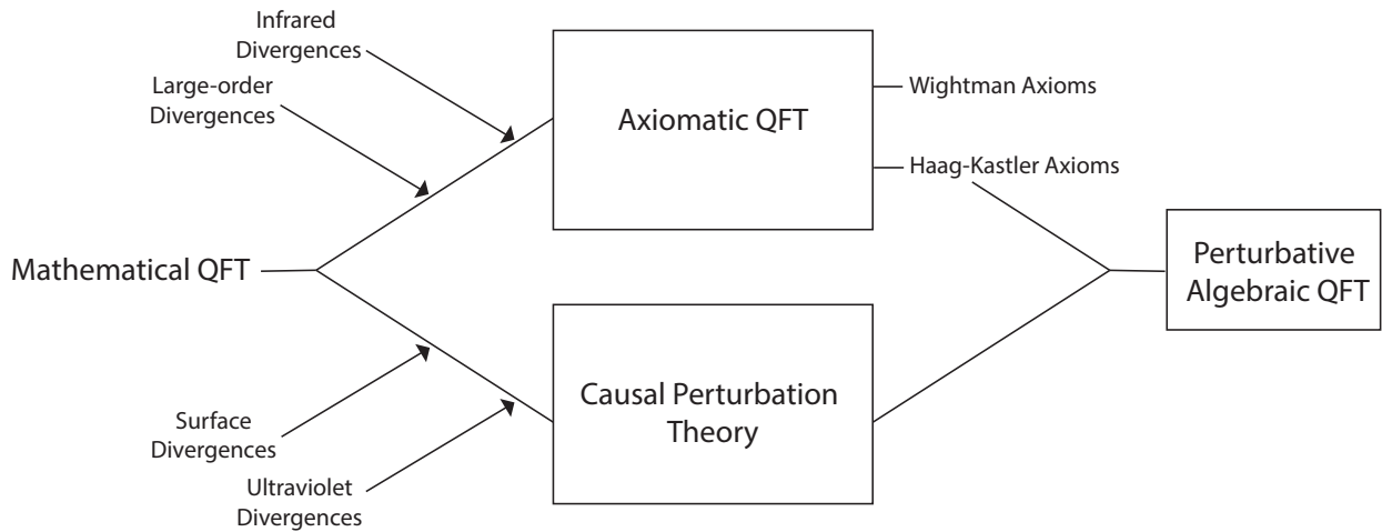
Figure 2: Continuation of Figure 1, depicting perturbative algebraic QFT (pAQFT) as bringing the earlier strands of axiomatic QFT and causal perturbation theory together.
