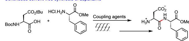
Scheme 1. Previously reported syntheses of peptides by twin-screw extrusion and outline of this work. Generic twin screw extruder symbol:
