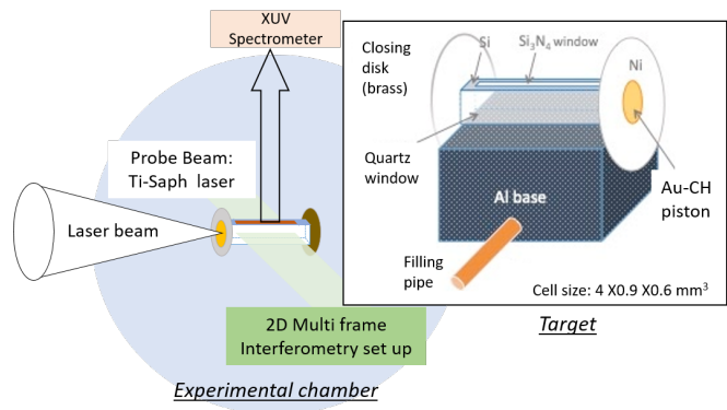
FIG. 1. Layout of the experimental setup and target (in the inset). The laser beam (0.3 ns, 100-180 J, 430 nm) focuses on the CH layer of the Au-CH piston of the target. An XUV spectrometer looks from the top through the SiN window of the target. The direction of the Ti-Saph probe beam for the 2D interferometry is presented in the schematic in green colour. It propagates through the two lateral quartz windows.
