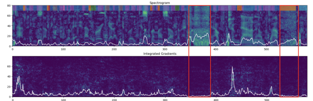
Figure 3: Spectrogram of an utterance from VoxCeleb1 (top), it's associated integrated gradients (bottom), and the phoneme segmentation colored by category of phonemes (upper part). Red boxes show parts with no phonemes detected. In white is the power of the spectrogram and the integrated gradients.
