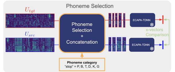
Figure 1: Illustration of the phoneme selection for computing the x-vectors from specific phoneme categories.
