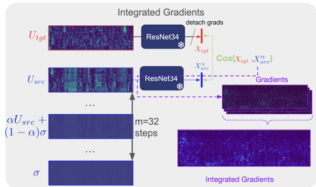
Figure 2: Computation of integrated gradients on a frozen speaker verification system, given a couple of utterances U_{src} and U_{tgt} from the same speaker, using m = 32 steps for the Riemann's integral.
