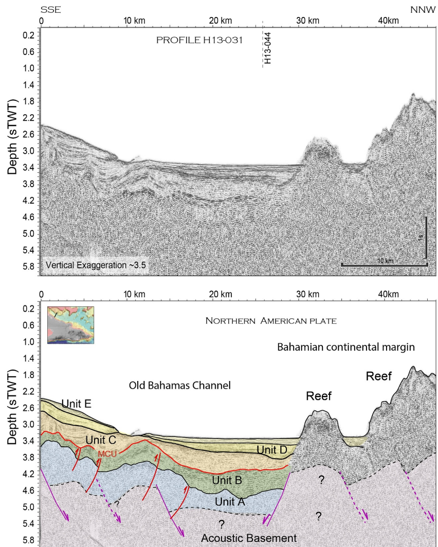
Figure 11. Seismic line H13-031. Seismic profile crossing the Old Bahamas Channel from SSE to NNW. MCU: Mid-Cretaceous Unconformity. See the inset and Figure 4a for the location of the profile.
