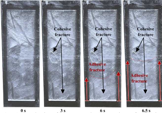
Fig. 15. Cohesive fractures and propagation of adhesive fracture at the 3 rd extension mode.
