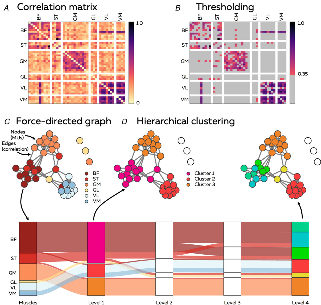
Figure 3. Construction of the correlation networks of spinal motor neurons
