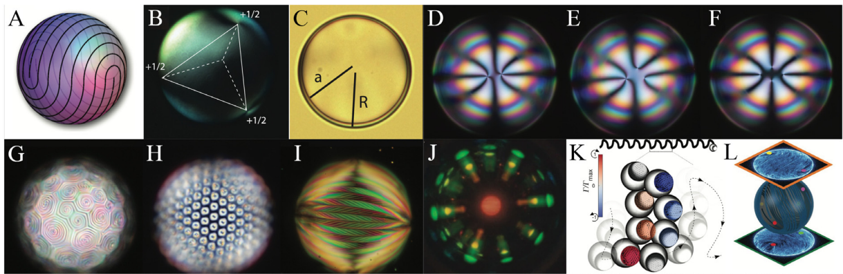
Fig. 74. A Two-dimensional spherical nematic with four +1/2 disclinations organized in a tetrahedral fashion. B Experimental nematic shell reproducing the tetrahedral defect structure shown in A . C Double emulsion with an inner radius a , an outer radius R , and an average thickness h = R - a . D–F Defect configurations in nematic shells with planar anchoring and thickness heterogeneity: D bivalent configuration with two pairs of +1 boojums on each spherical boundary, E trivalent configuration with a +1 boojum on each spherical boundary and two +1/2 disclinations that span the shell, and F tetravalent configuration with four +1/2 disclinations spanning the shell. G Cholesteric shell with hybrid boundary conditions displaying double-spiralled thin stripes inside focal conic domains. H Cholesteric shell with homeotropic anchoring showing a close-packed structure of axisymmetric topological solitons. I Smectic shell with planar boundary conditions, where curvature walls divide the sphere into crescent domains. J Photonic cross communication patterns in a cholesteric shell. K Swimming trajectory of a self-propelled nematic shell with homeotropic boundary conditions. L Two dimensional active nematic shell, where microtubule bundles are sheared by kinesin motors. The two projections show the positions of the four +1/2 disclinations, which continuously oscillate over time. B and D–J are crossed polarized images, while C is a bright-field image. The typical outer radii of the passive shells are around 100\ \mu\text{m} , the active shell is five times smaller.
