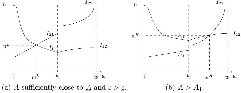
Figure 5: Existence and uniqueness of a steady state
