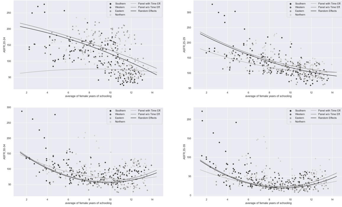
Figure 4: Predicted values.
