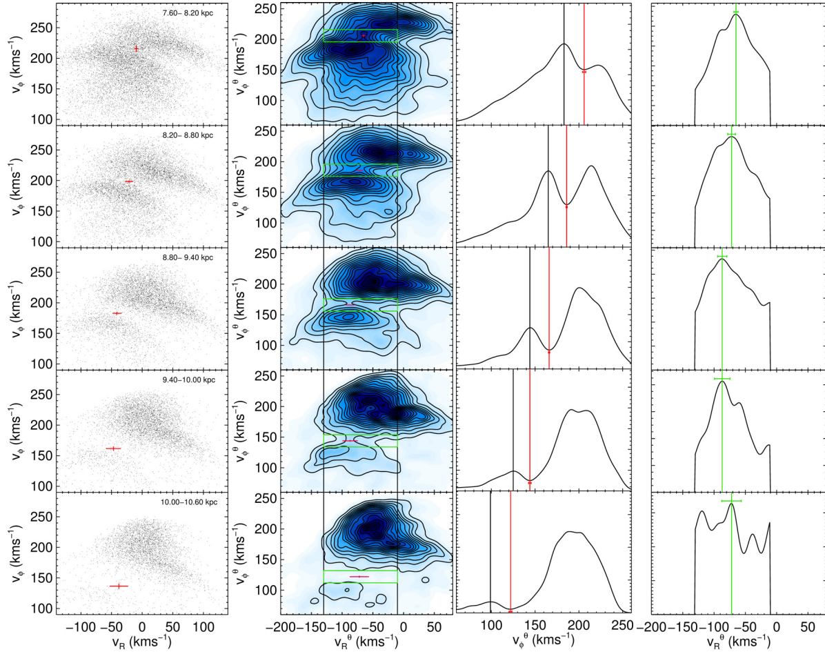
Fig. 5. Illustration of the steps followed to locate the saddle point v_{\phi,\text{OLR}} for the band at 40 deg. First column: scatter plot of the velocities in bins in radius as indicated in the top right part of the panels. The red cross in these panels shows our determination of the saddle point. Second column: velocity distribution computed with the kernel adaptive method after a rotation of coordinates by an angle \theta = 15 deg. Third column: distribution of v_{\phi}^{\theta} inside the region limited by black vertical lines shown in the second column. The red vertical line and red error bar show the position of the minimum corresponding to the v_{\phi}^{\theta} velocity of the saddle point and its error e_{\text{bst}} . The black vertical line indicates the Hercules peak. Fourth column: distribution in v_R^{\theta} inside the green rectangle shown in the second column. The green vertical line and green error bar shows the position of the maximum which corresponds to the v_{R,\text{OLR}}^{\theta} velocity of the saddle point and its error e_{\text{bst}} .
