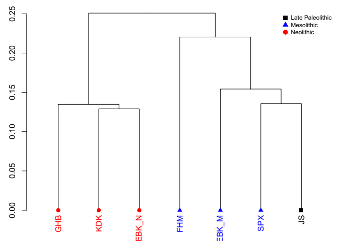
FIGURE 3 Ward's minimum variance agglomerative clustering dendrogram based on the size-corrected crown measurements of seven Nile Valley samples (see Table 1 for site abbreviations). EBK_M, Mesolithic El-Barga; EBK_N, Neolithic El-Barga; FHM, Mesolithic Fox Hill; GHB, Ghaba; JS, Jebel Sahaba; KDK, Kadruka; SPX, Sphinx.
